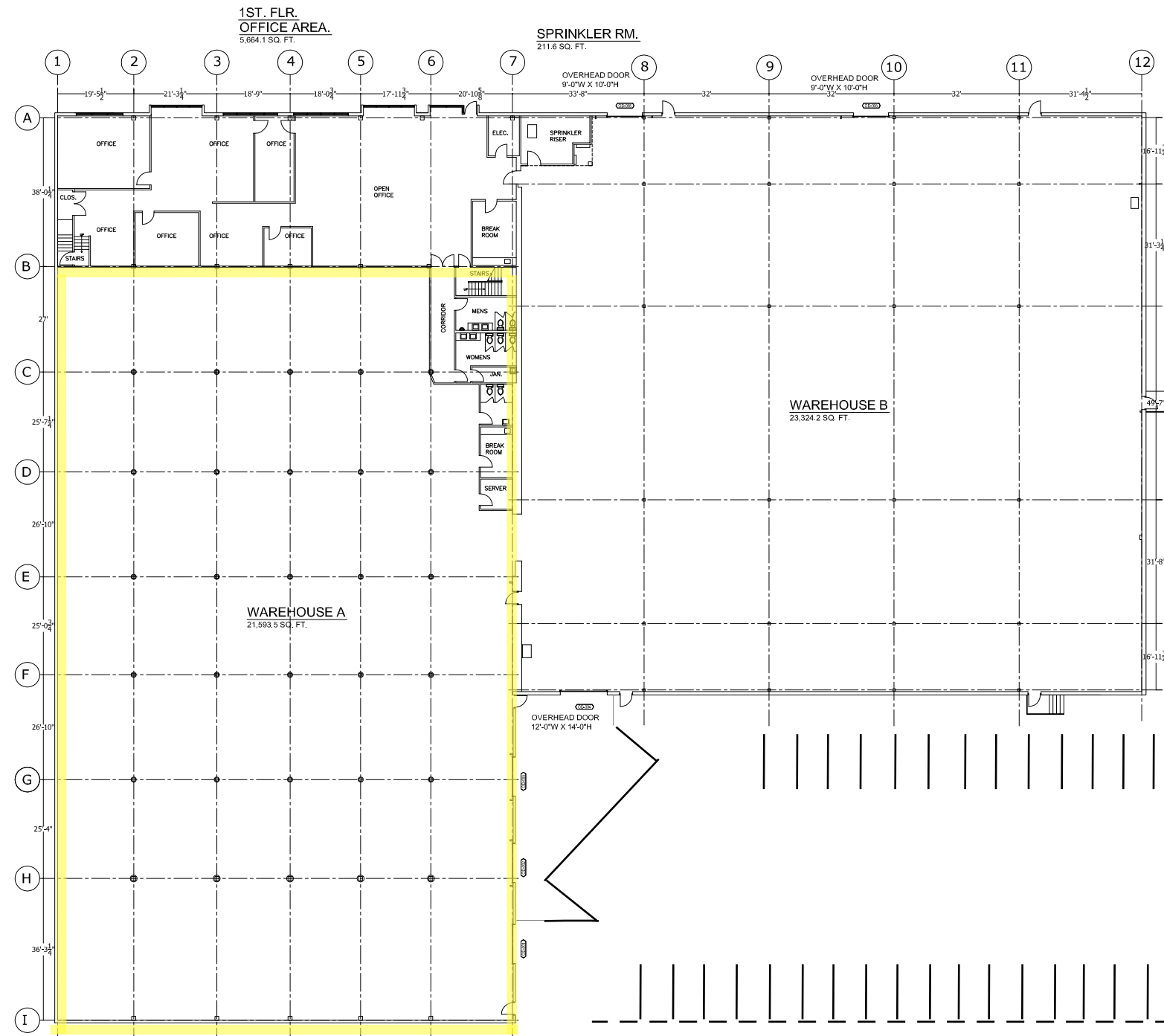
FIRST FLOOR PLAN IRON MOUNTAIN 1201 N. 96TH. ST. SEATTLE, WA
