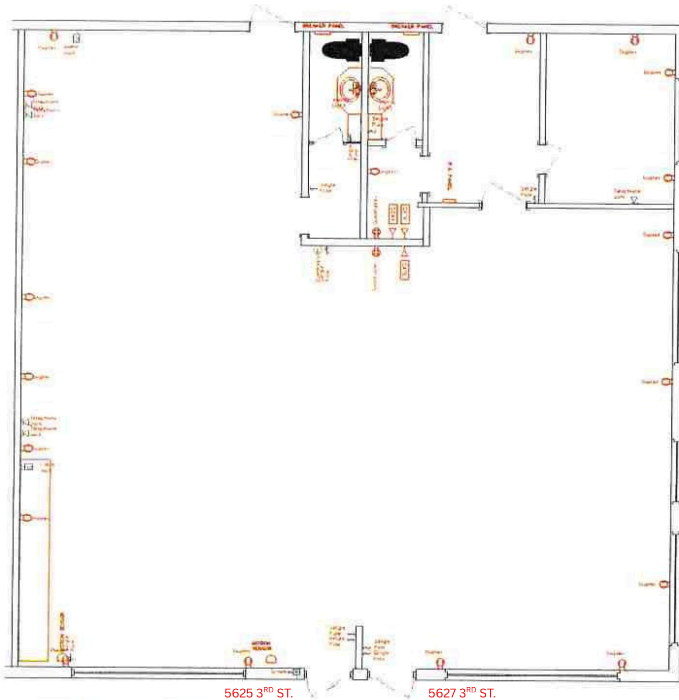
2 ELECTRICAL PLAN--(COMPLETED) SCALE: 1/4"=1'-0"
