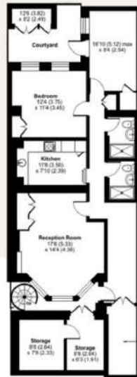
LOWER GROUND FLOOR FLAT 1
