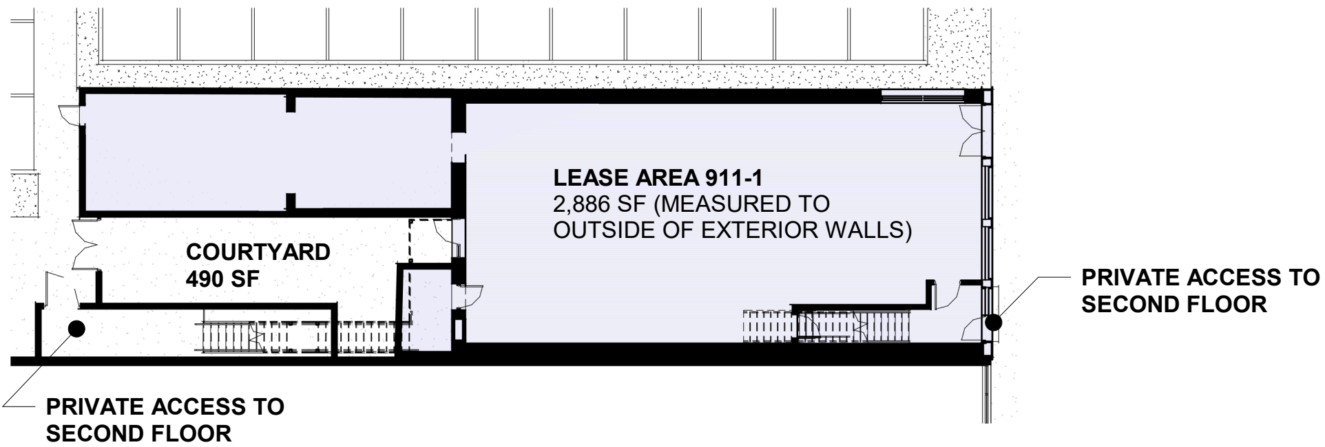
② FIRST FLOOR 911 GERVAIS LEASE AREA PLAN 1/16" = 1'-0"
