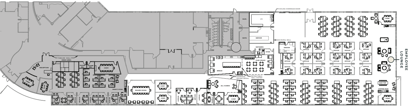
Furniture Plan
