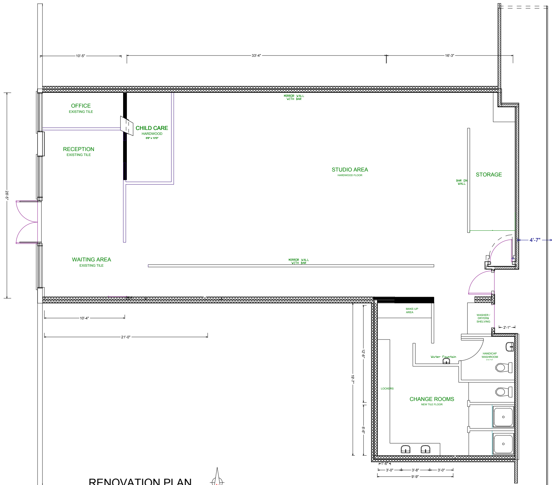
RENOVATION PLAN SCALE 1/4"=1'-0"
