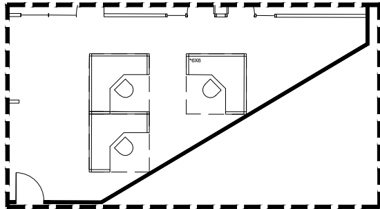
ALTERNATE OPEN OFFICE CUBE LAYOUT
