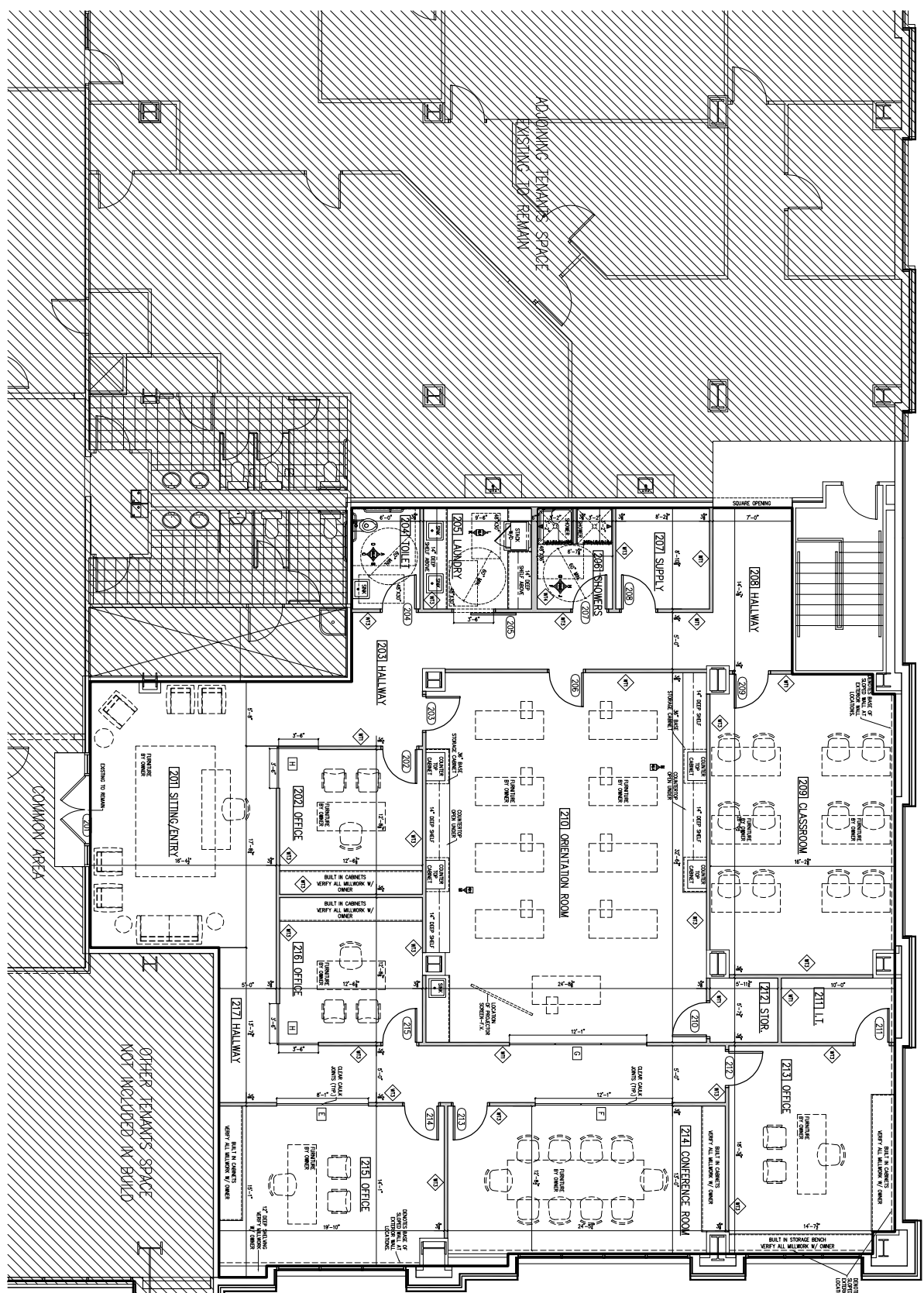
NEW TENANT FLOOR PLAN SCALE: 1/4" = 1'-0"
