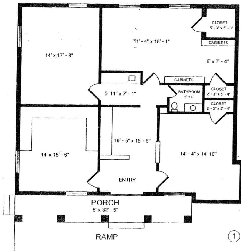
SUITE 100 FLOOR PLAN | 1,415 SF
