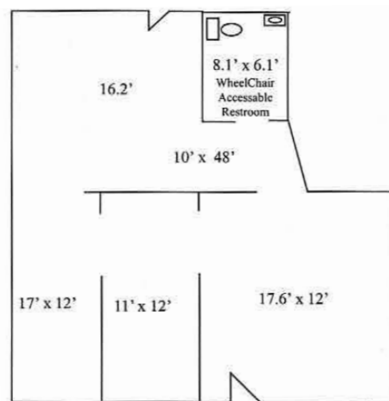
SUITE 200A FLOOR PLAN | 1,200 SF
