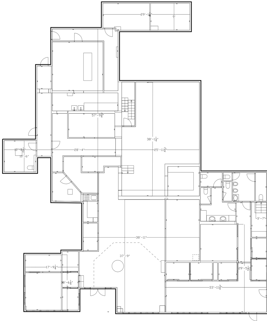
GROUND FLOOR 5,880 GSF*
