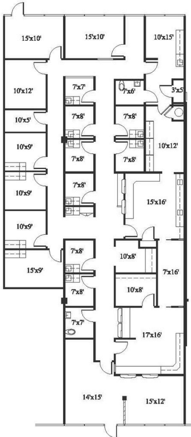
KEY PLAN
