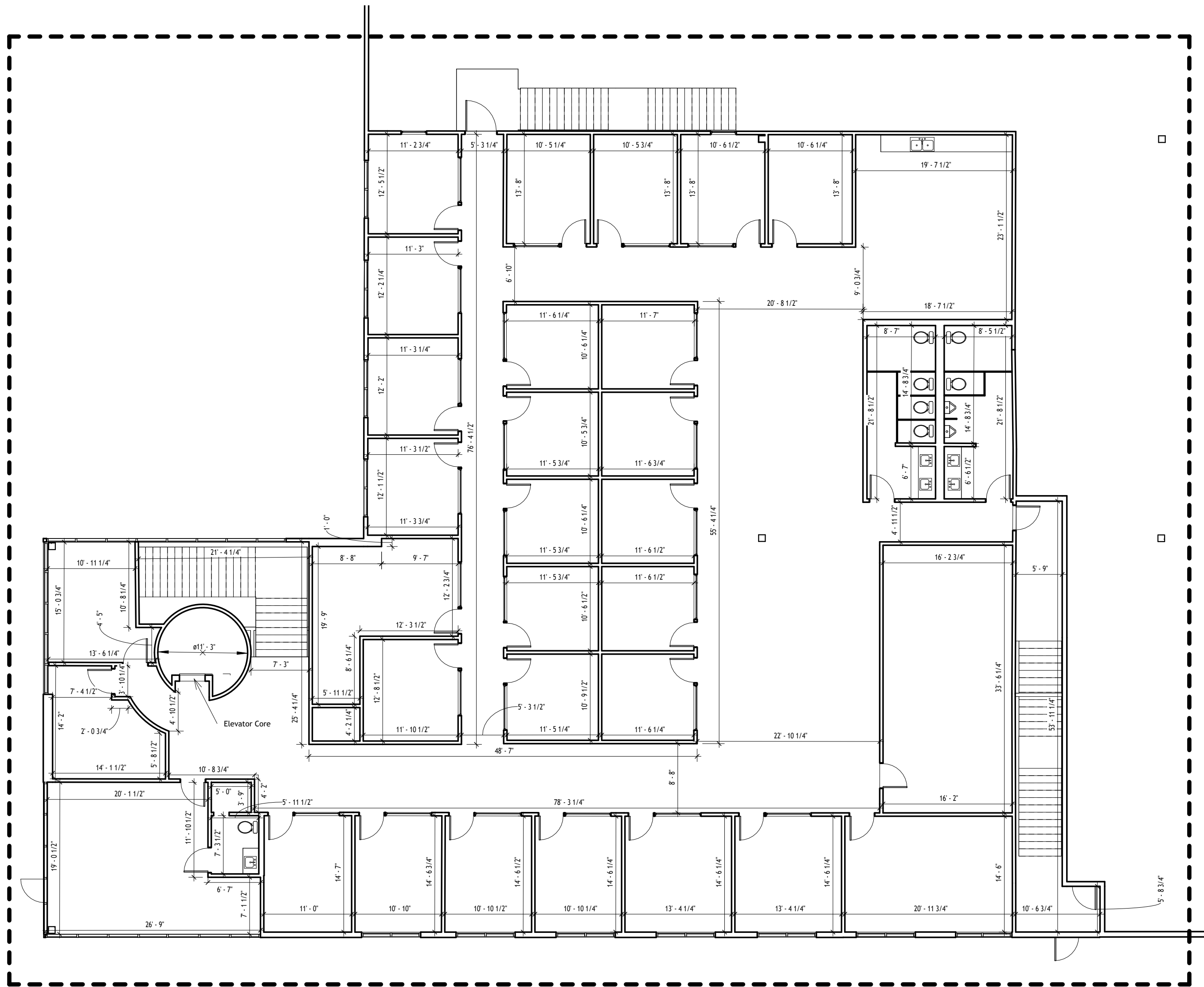
South Office Detail - Second Floor
