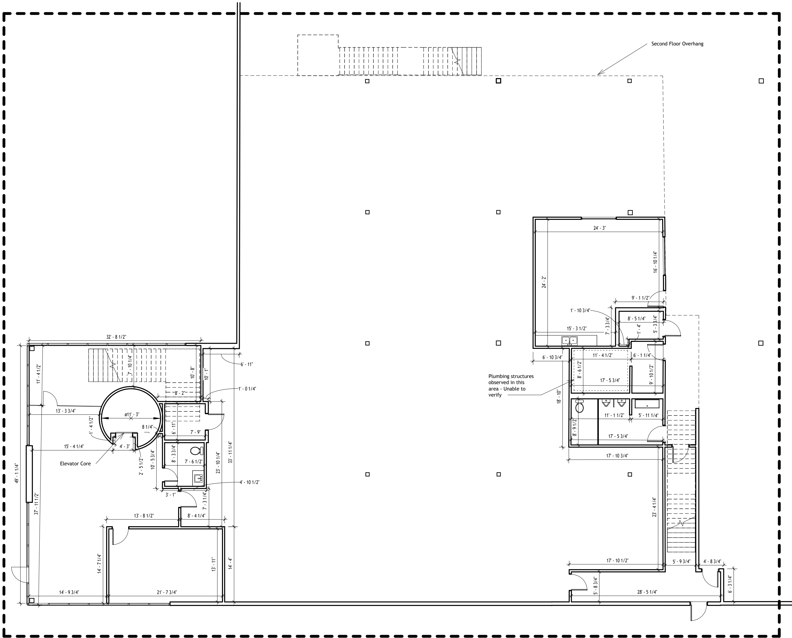
South Office Detail - First Floor
