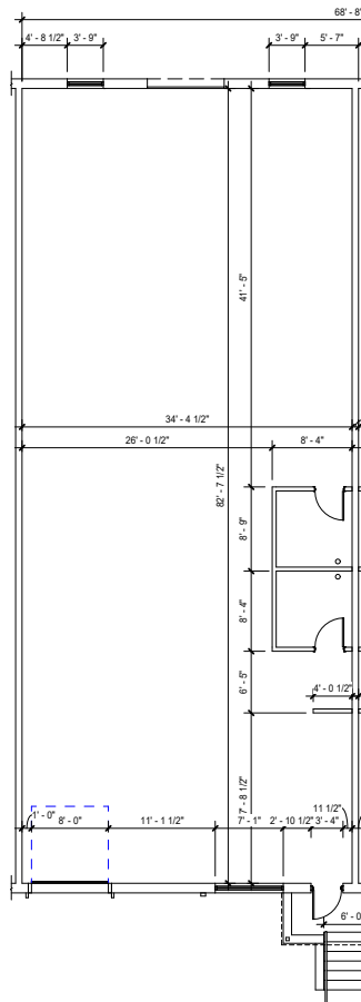
2 FIRST FLOOR DIMENSION PLAN - EXISTING 1/8" = 1'-0"
