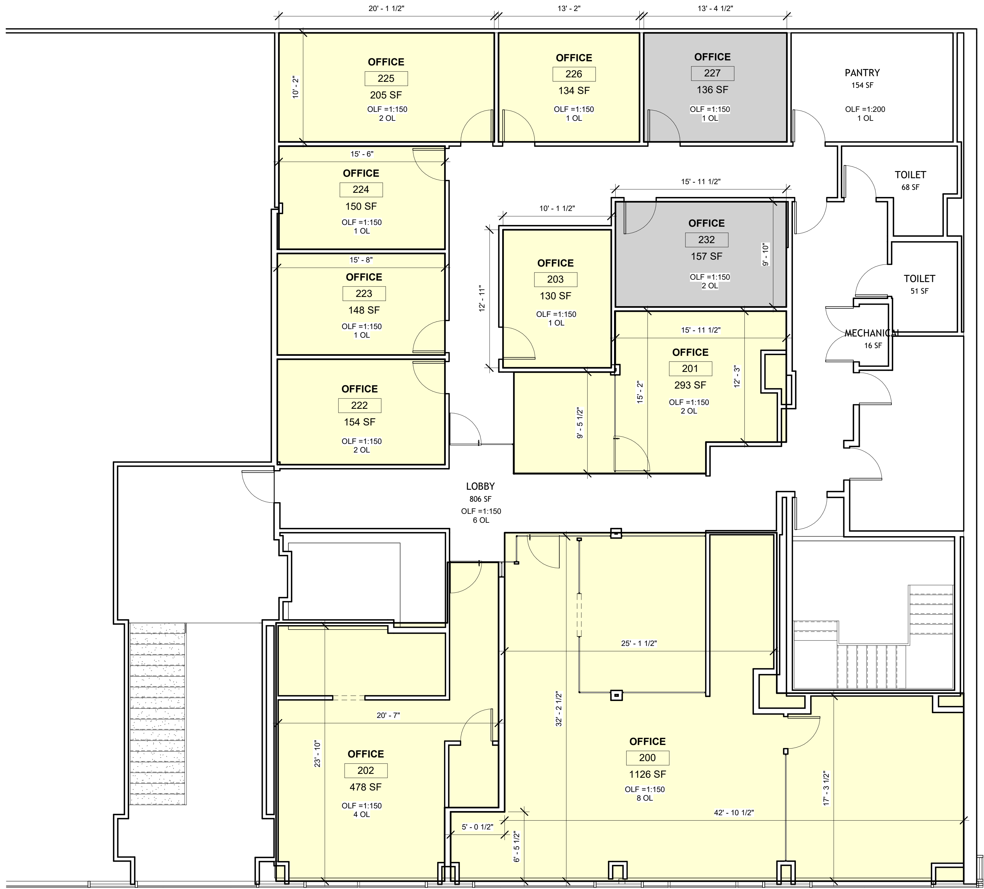
1 LEVEL 2 OFFICE AREA 3/16" = 1'-0"
