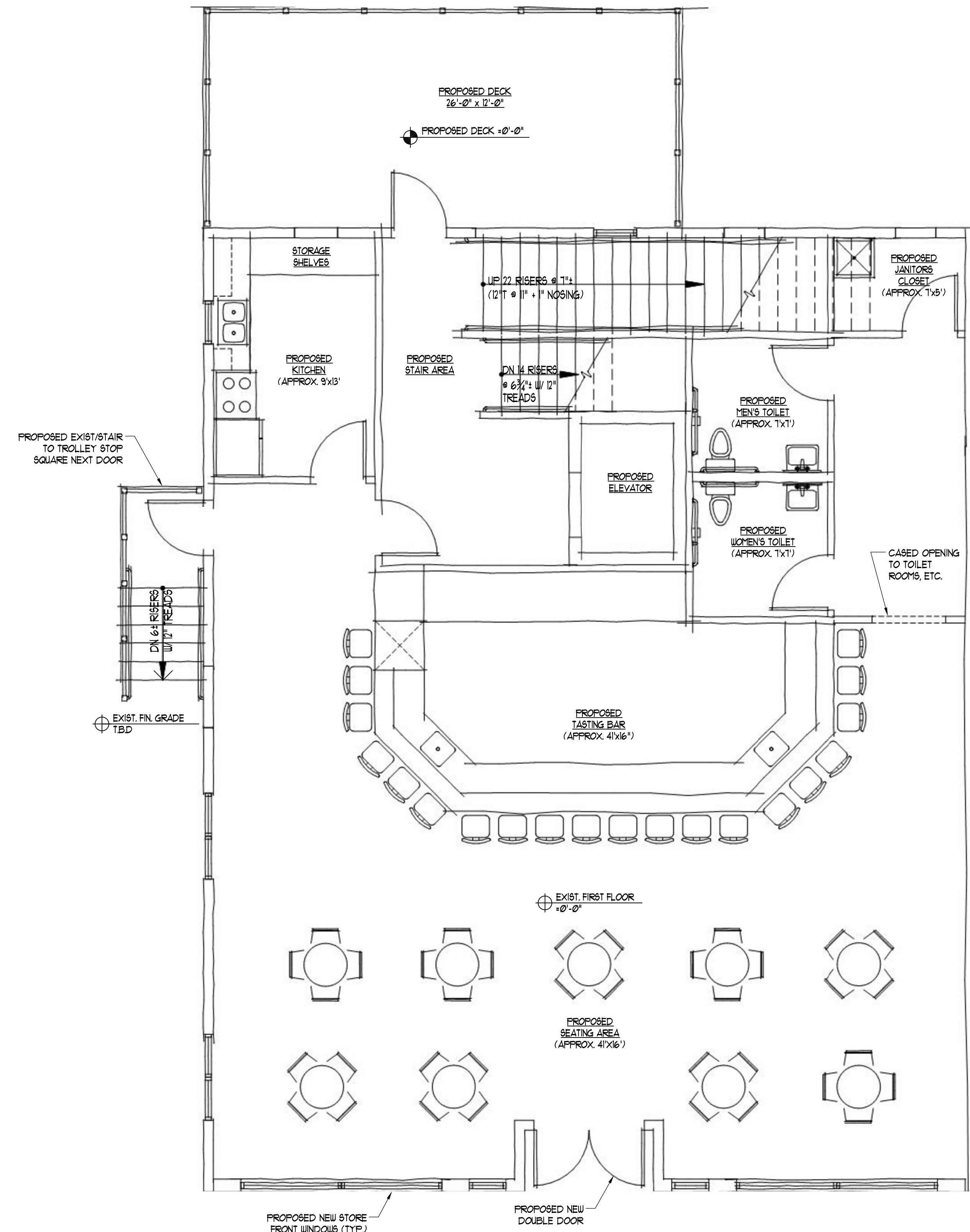
PROPOSED FIRST FLOOR RETAIL SPACE
