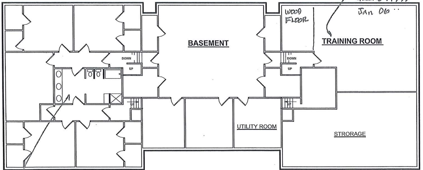
GROUND LEVEL
