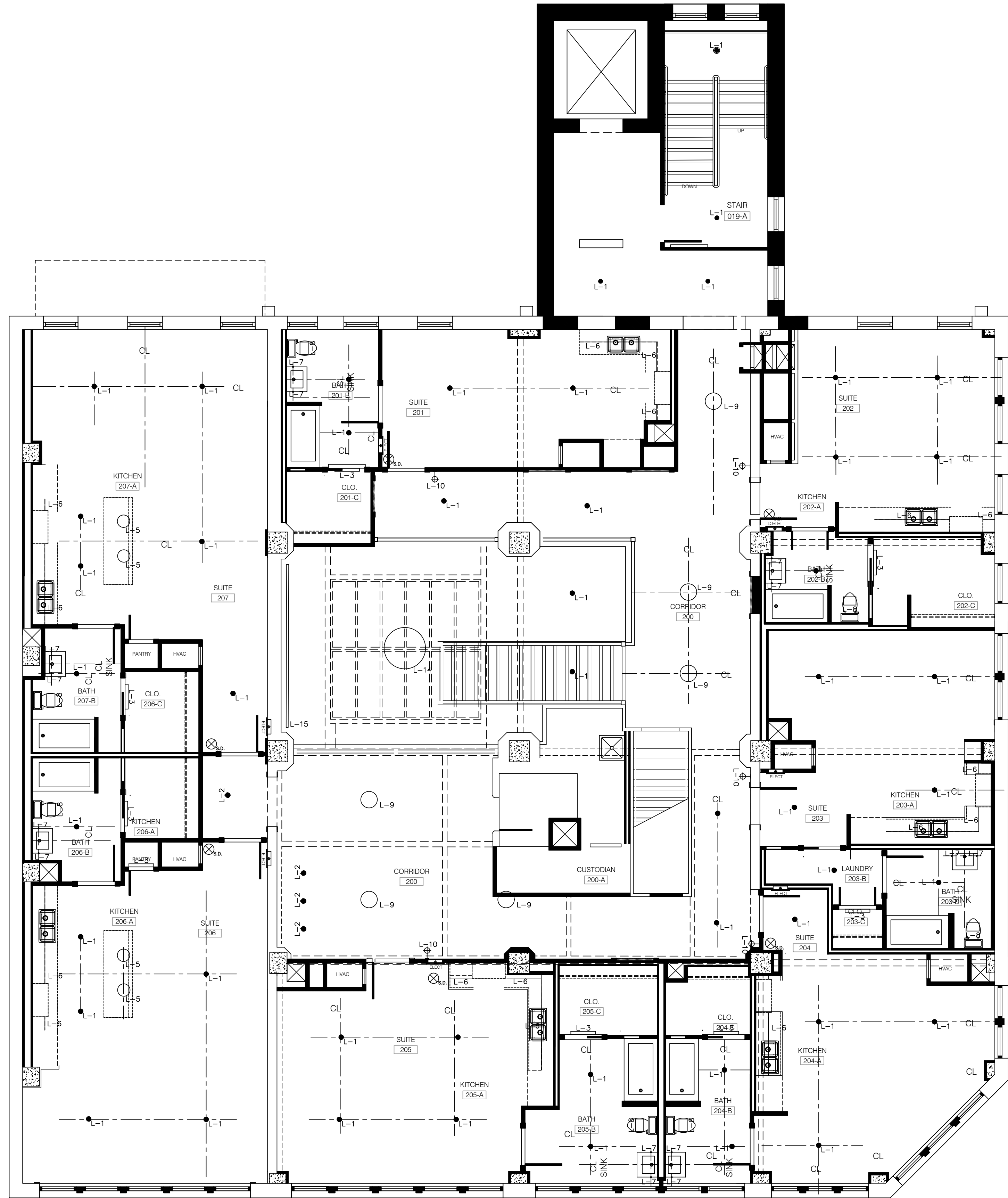
2nd FLOOR RCP SCALE: 3/16" = 1'-0"
