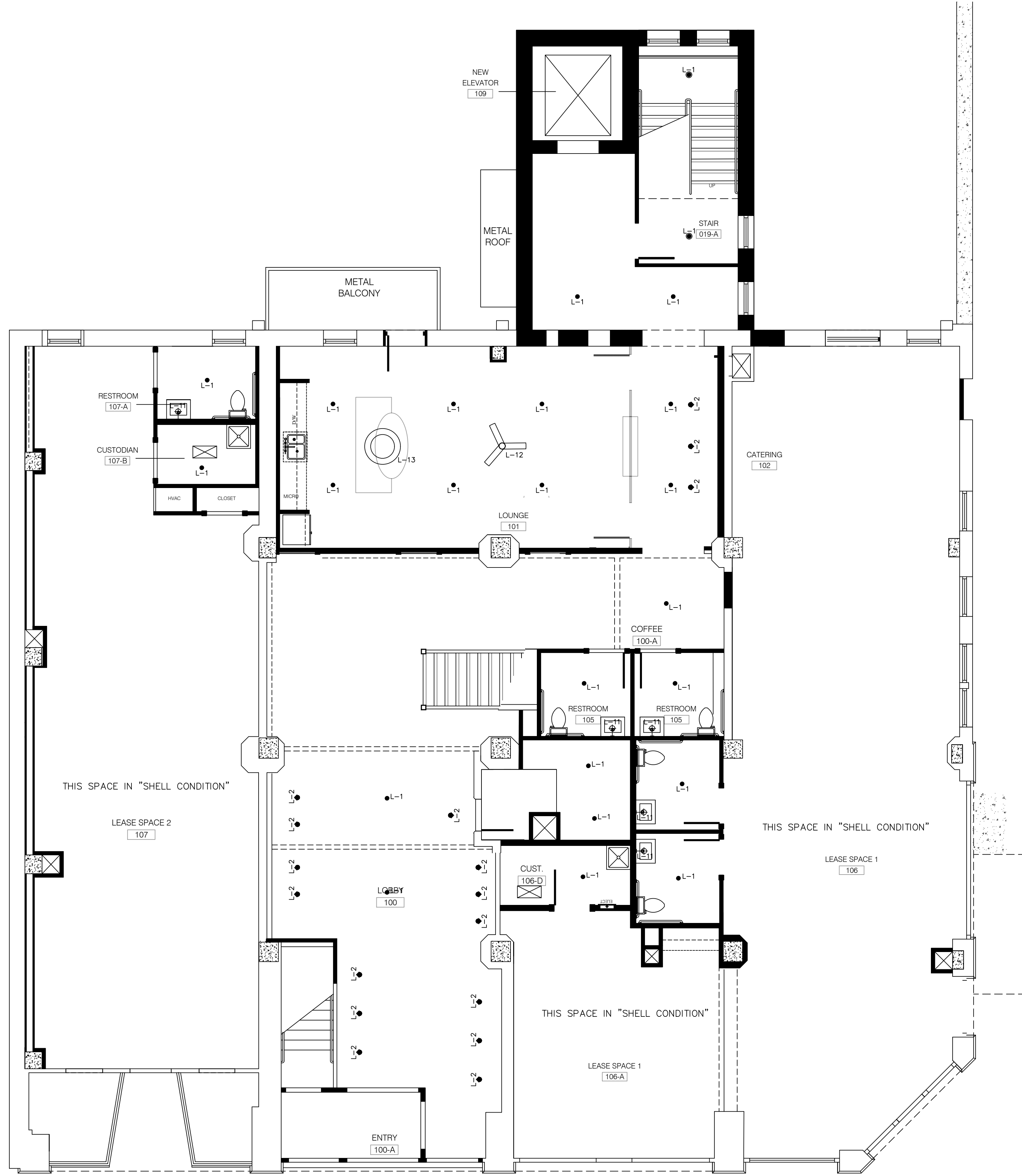
1st FLOOR RCP SCALE: 3/16" = 1'-0" 01
