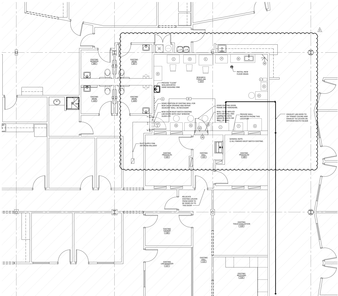
RESEARCH TISSUE LAB RENOVATION PLAN
