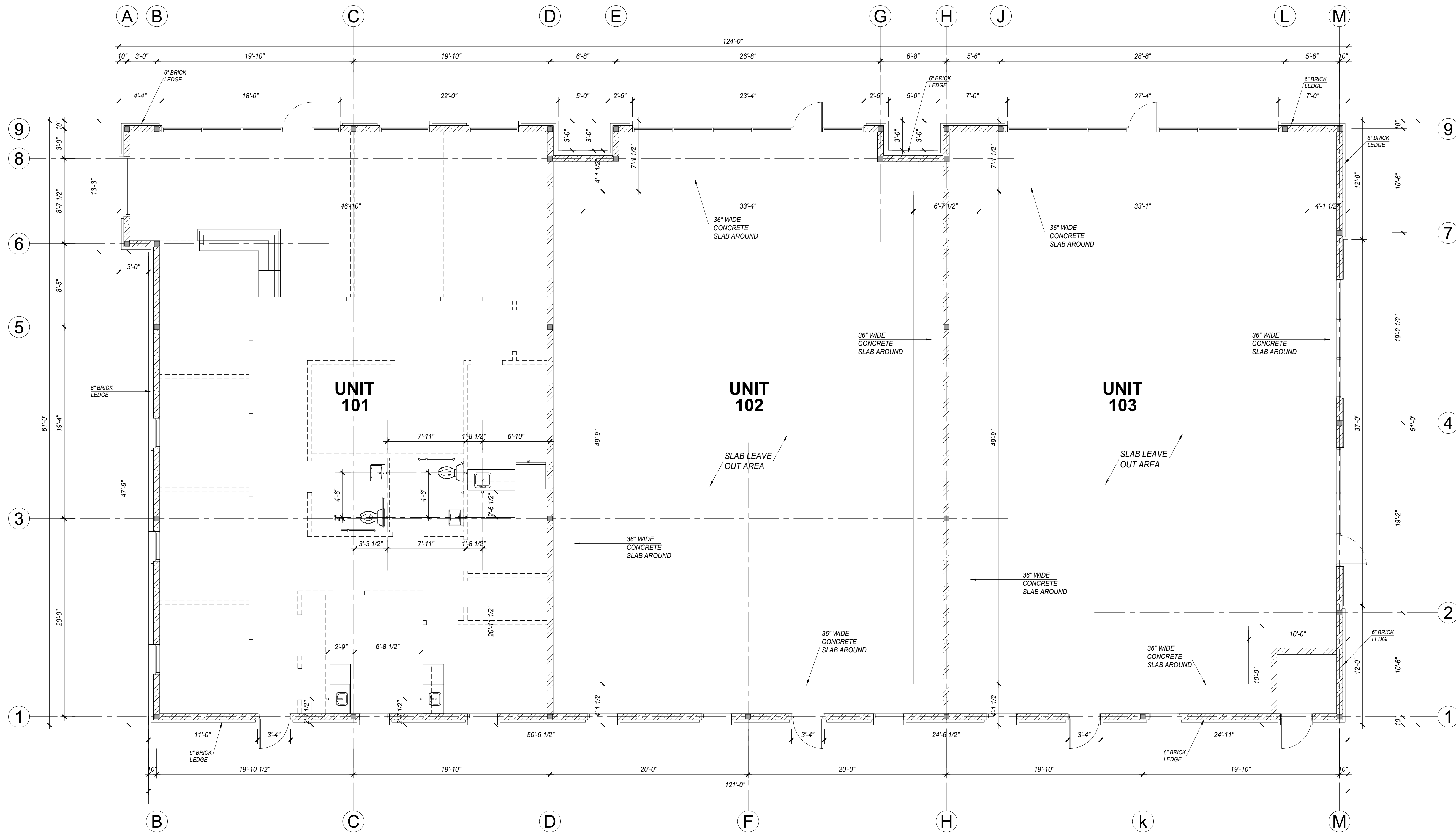
1 FIRST SLAB PLAN SCALE: 3/16"=1'-0"
