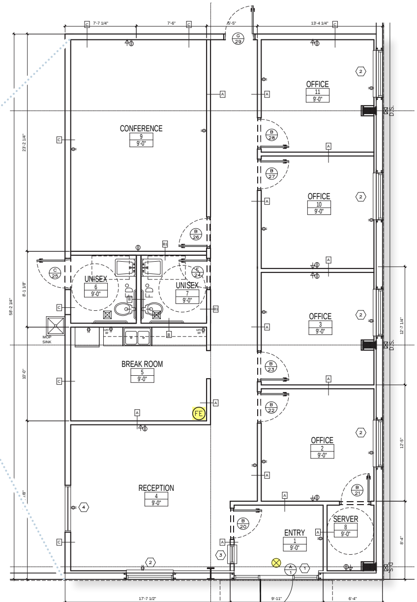
OFFICE PLAN | ±1,971 SF
