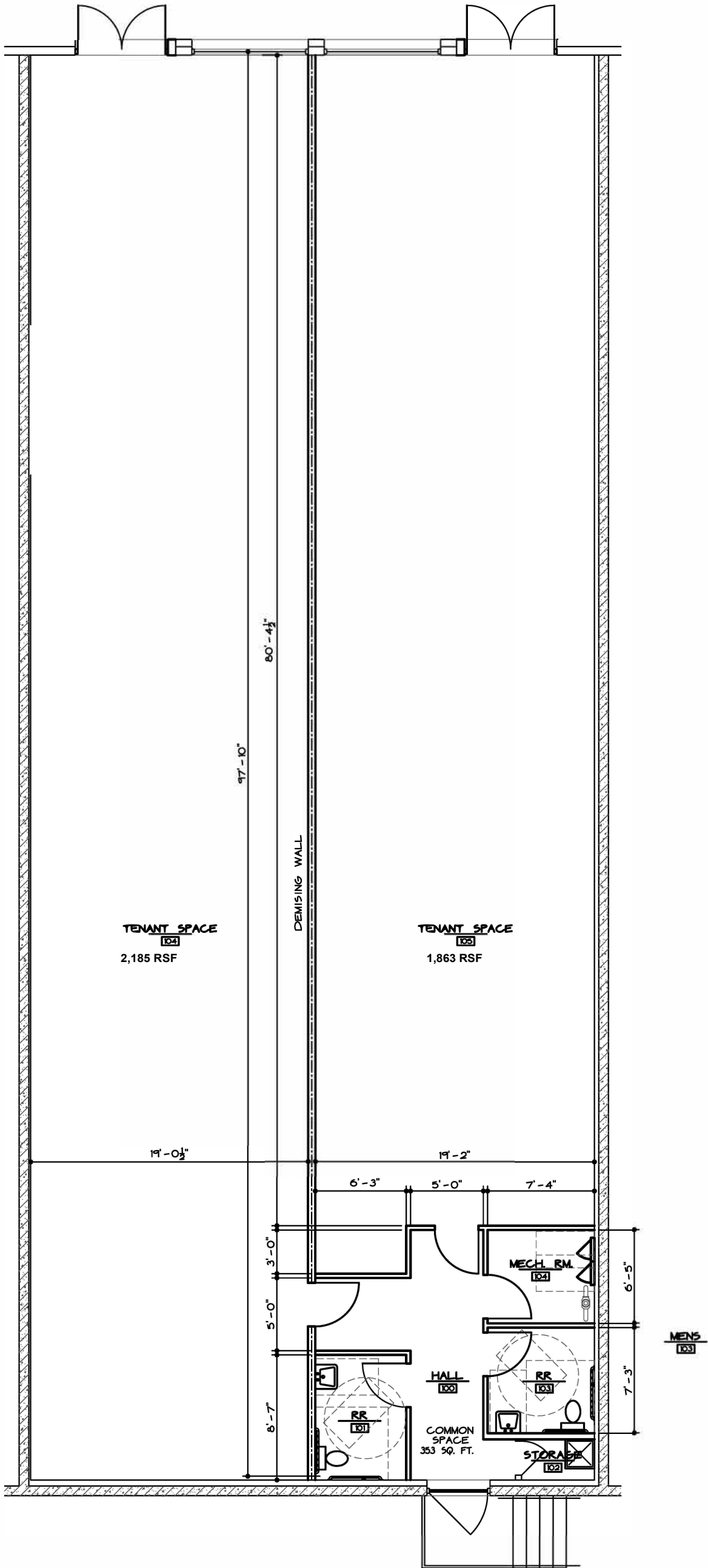
DEMOLITION FLOOR PLAN OPTION - 2
