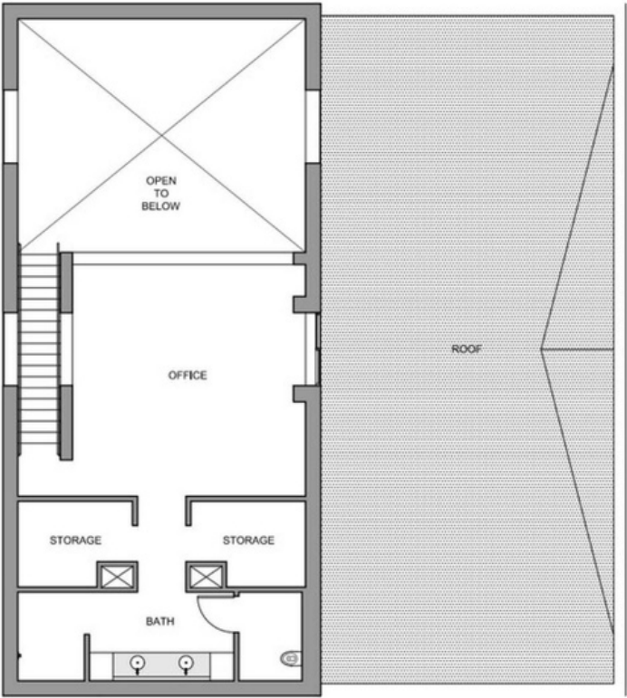
SECOND FLOOR - 958 SF
