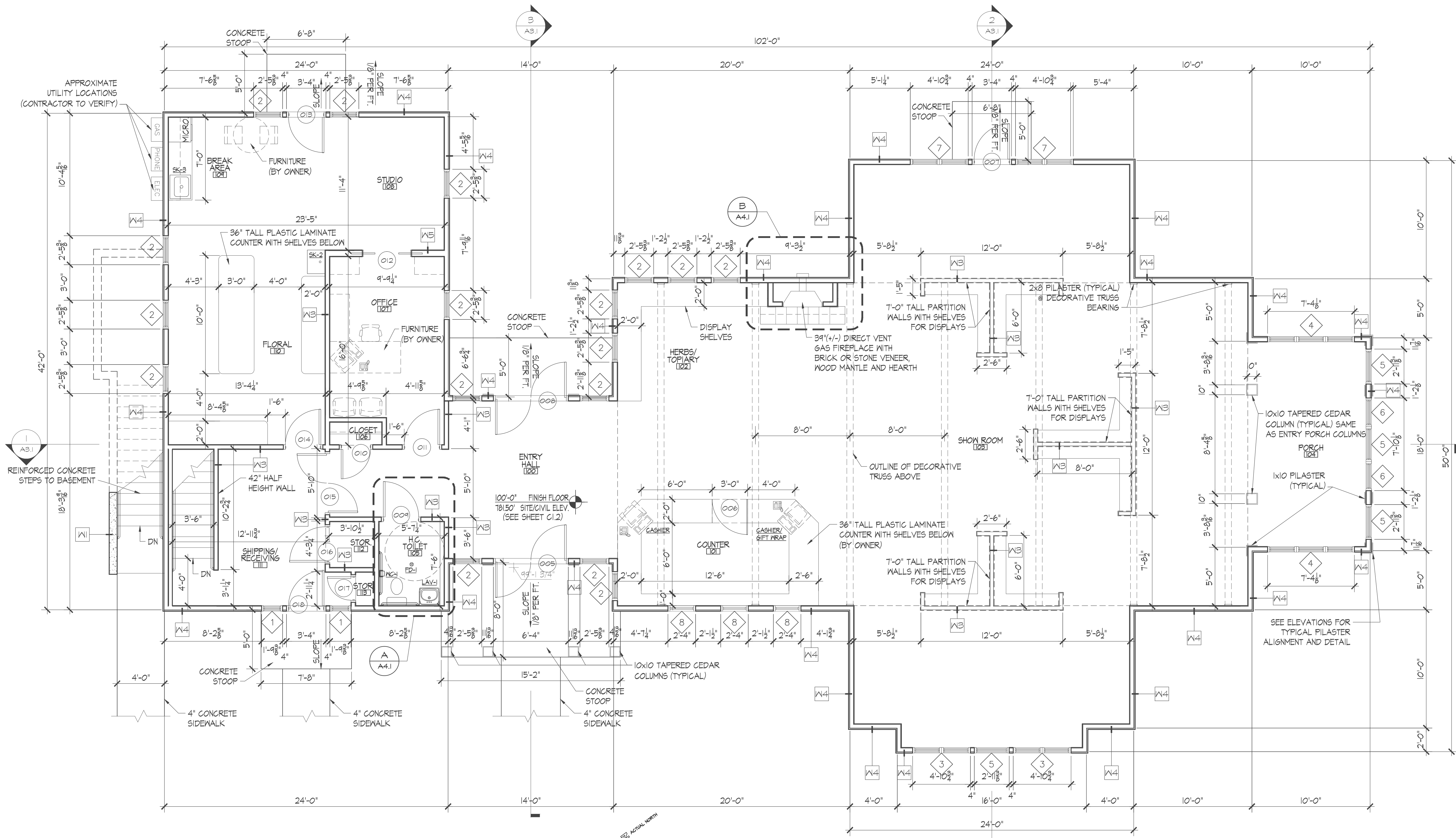
N PLAN NORTH FIRST FLOOR PLAN SCALE: 1/4" = 1'-0"
