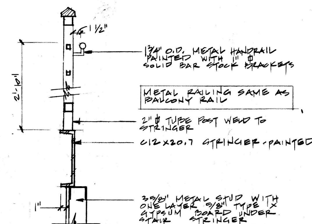
SECTION AT LOBBY STAIR 1/2" = 1'-0"
