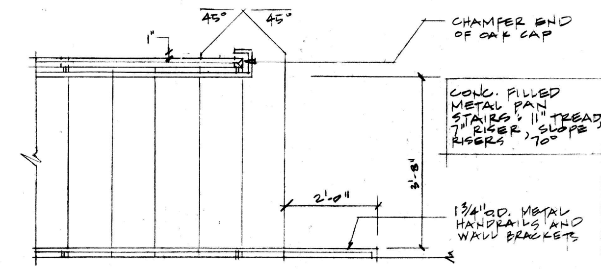
PLAN AT LOBBY STAIR 1/2" = 1'-0"
