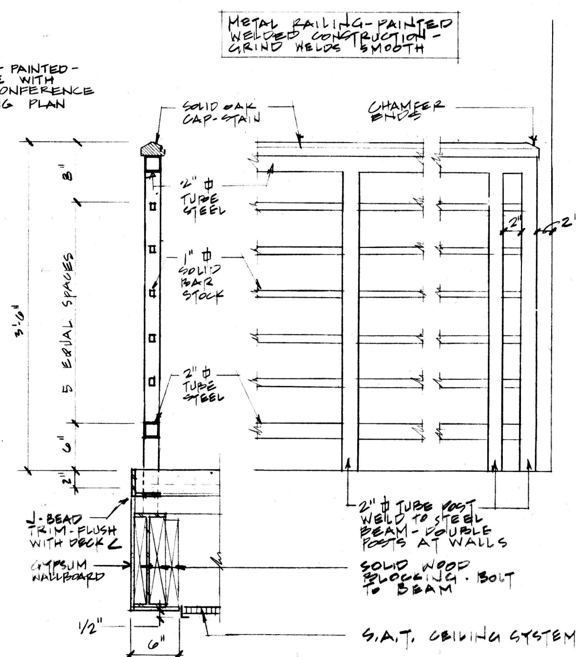
SECTION AND ELEVATION - BALCONY RAIL 1/2" = 1'-0"
