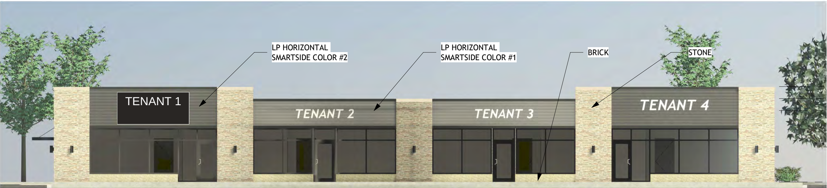
1 NORTH ELEVATION 1" = 10'-0"
