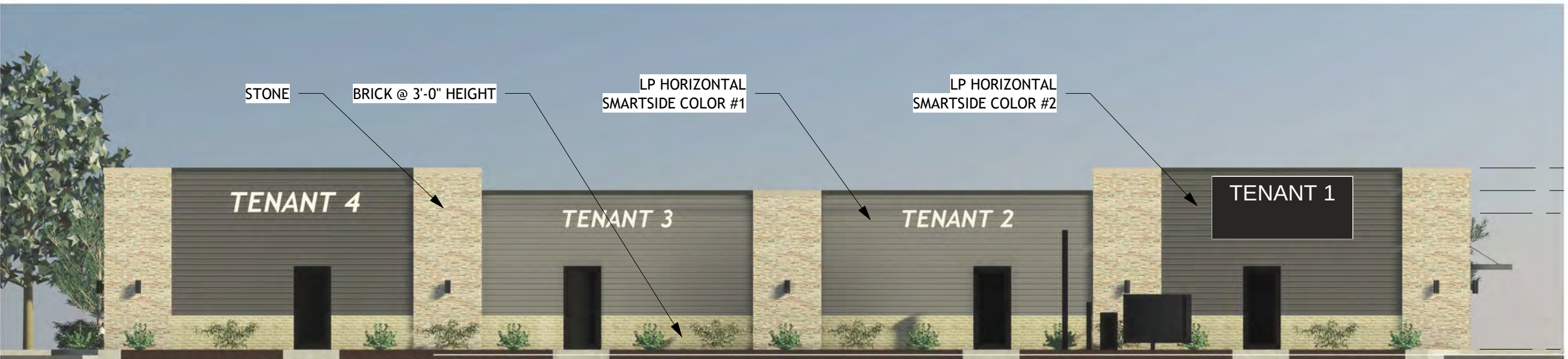
2 SOUTH ELEVATION 1" = 10'-0"
