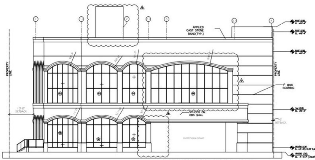
SOUTH ELEVATION -NE 28TH STREET
