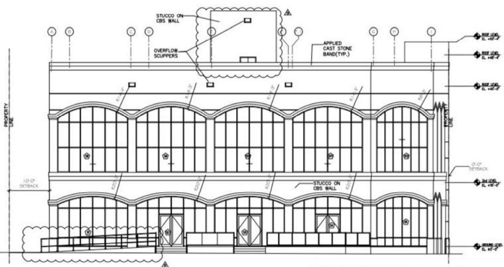
WEST ELEVATION -BISCAYNE BOULEVARD
