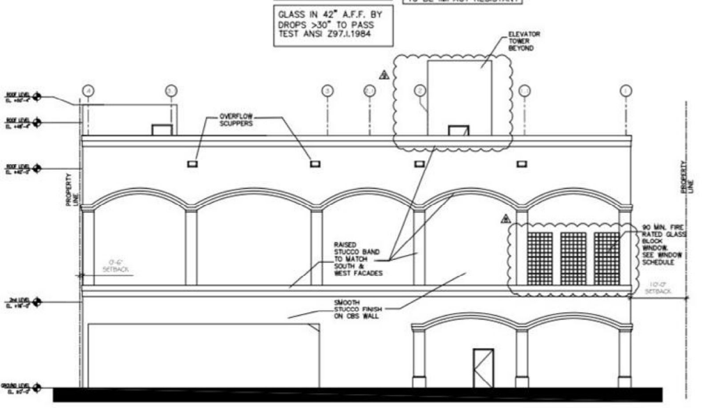
NORTH ELEVATION
