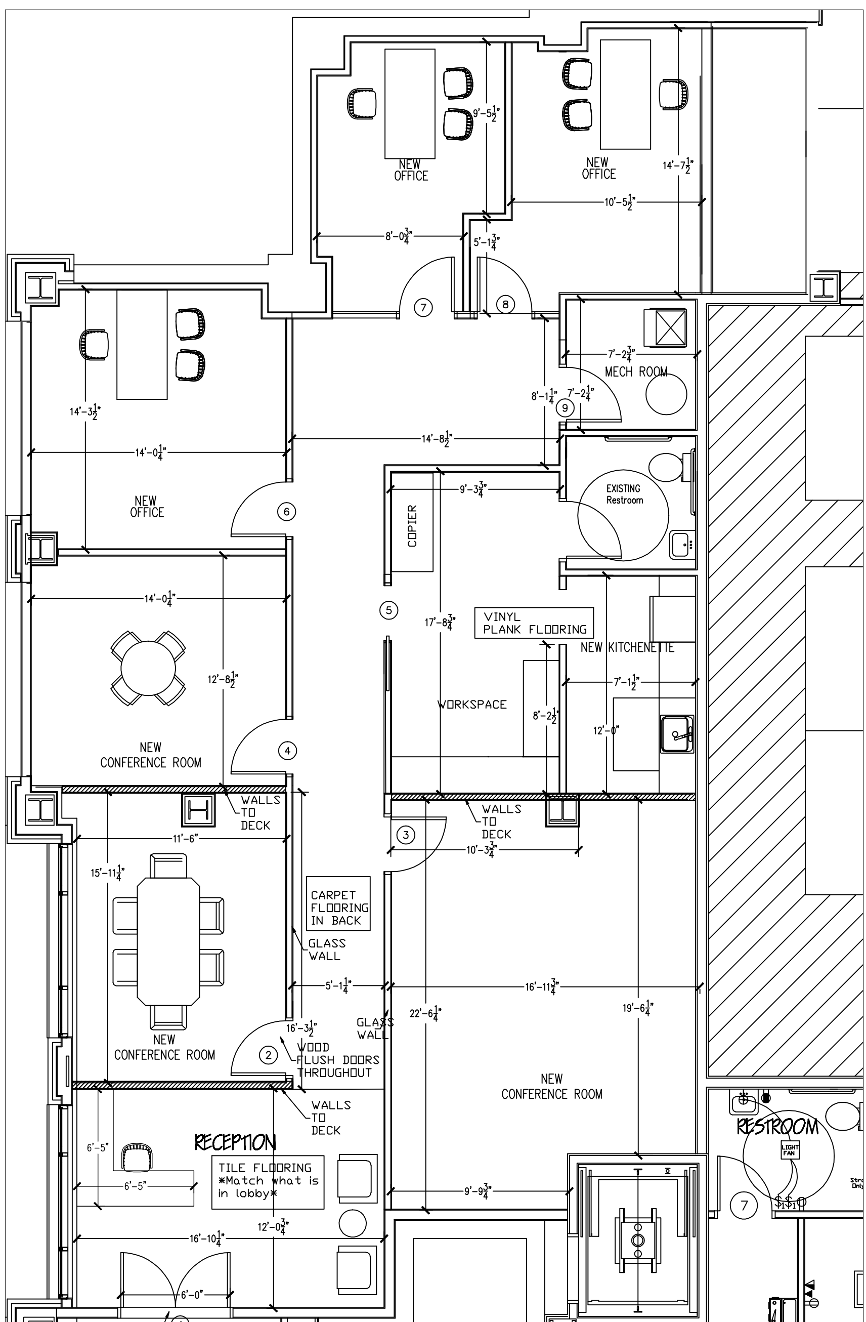
1 Park Place 104- Layout Plan 3/16" = 1'-0"
