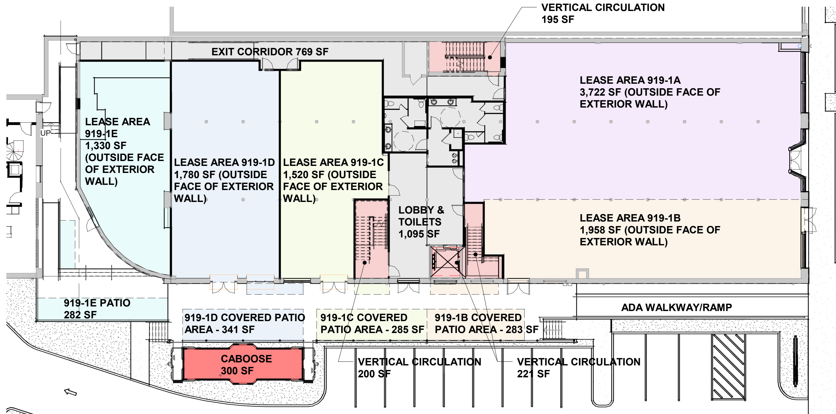
① 919 GERVAIS FIRST FLOOR LEASE AREA PLAN - OPTION 4 - COMMON TOILETS 1/16" = 1'-0"
