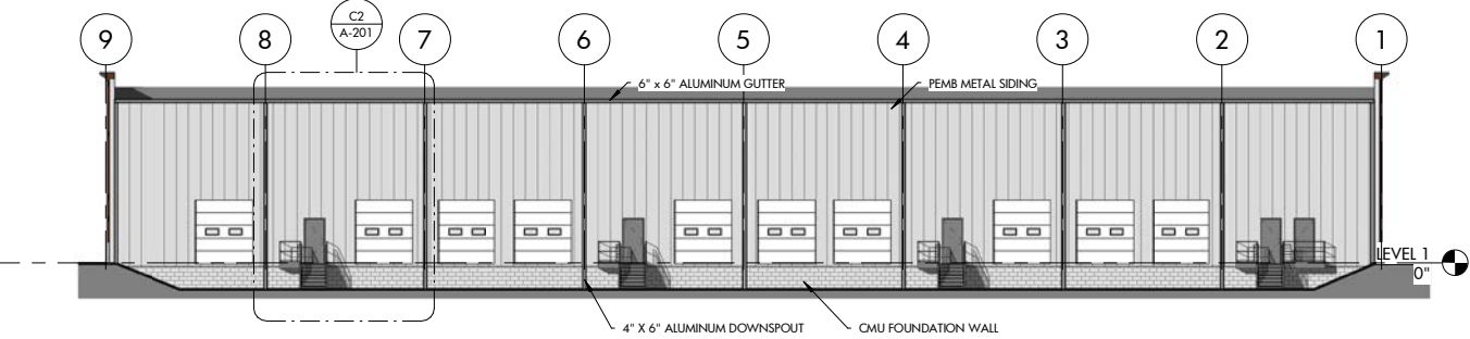
A1 NORTH ELEVATION A-201 1/16" = 1'-0"
