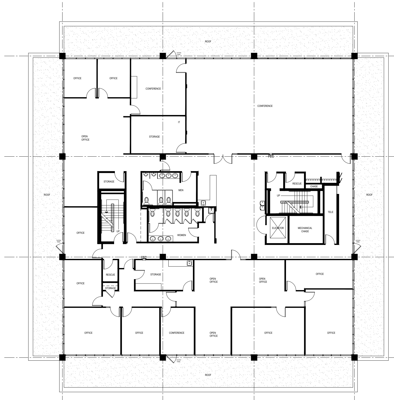
1 As-Built Floor Plan - Level 4
