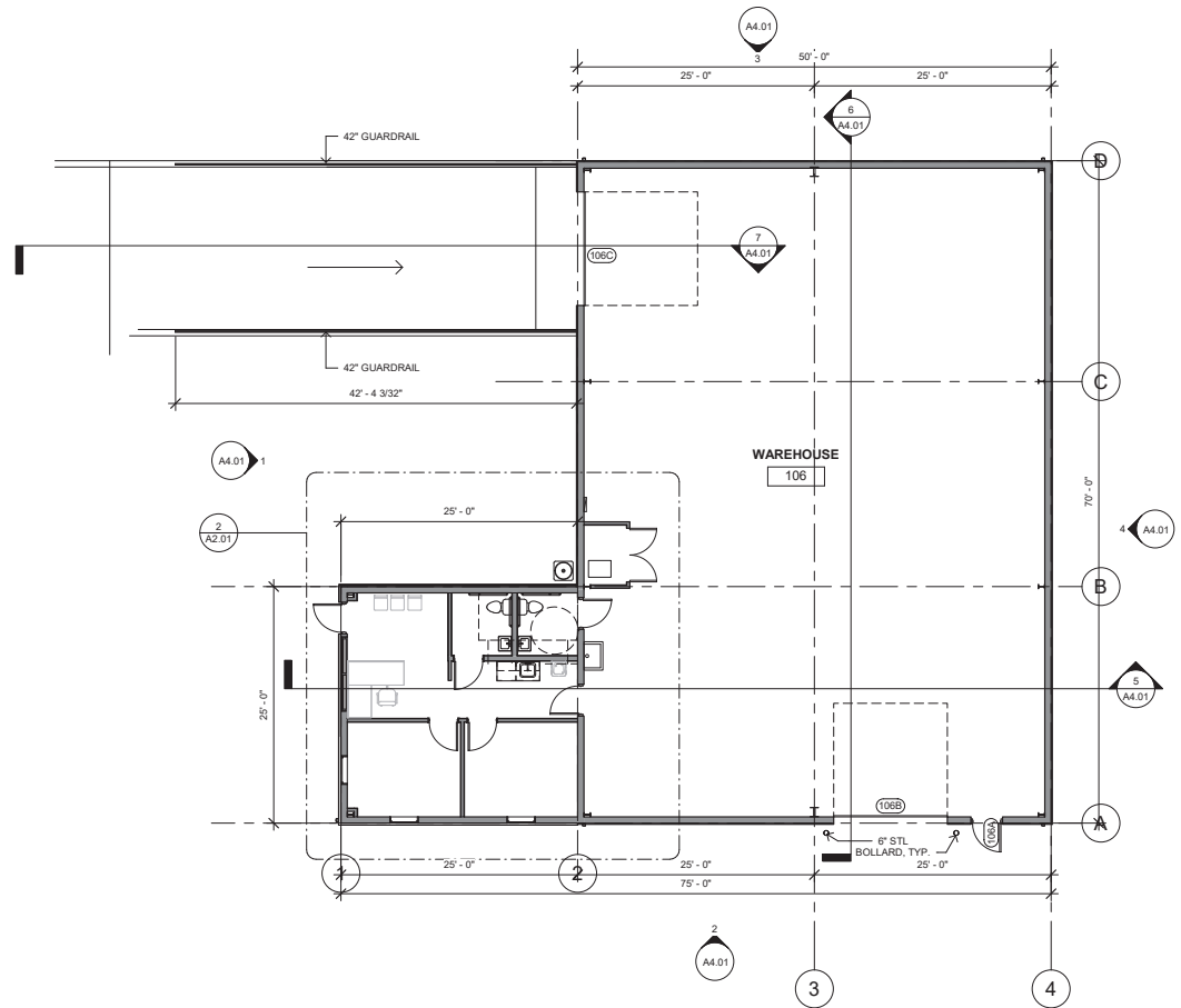
1 PROPOSED FLOOR PLAN 1/8" = 1'-0"
