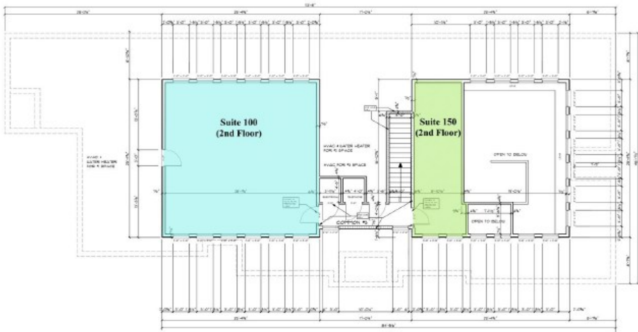
SECOND FLOOR PLAN SCALE: 1/4" = 1'-0"
