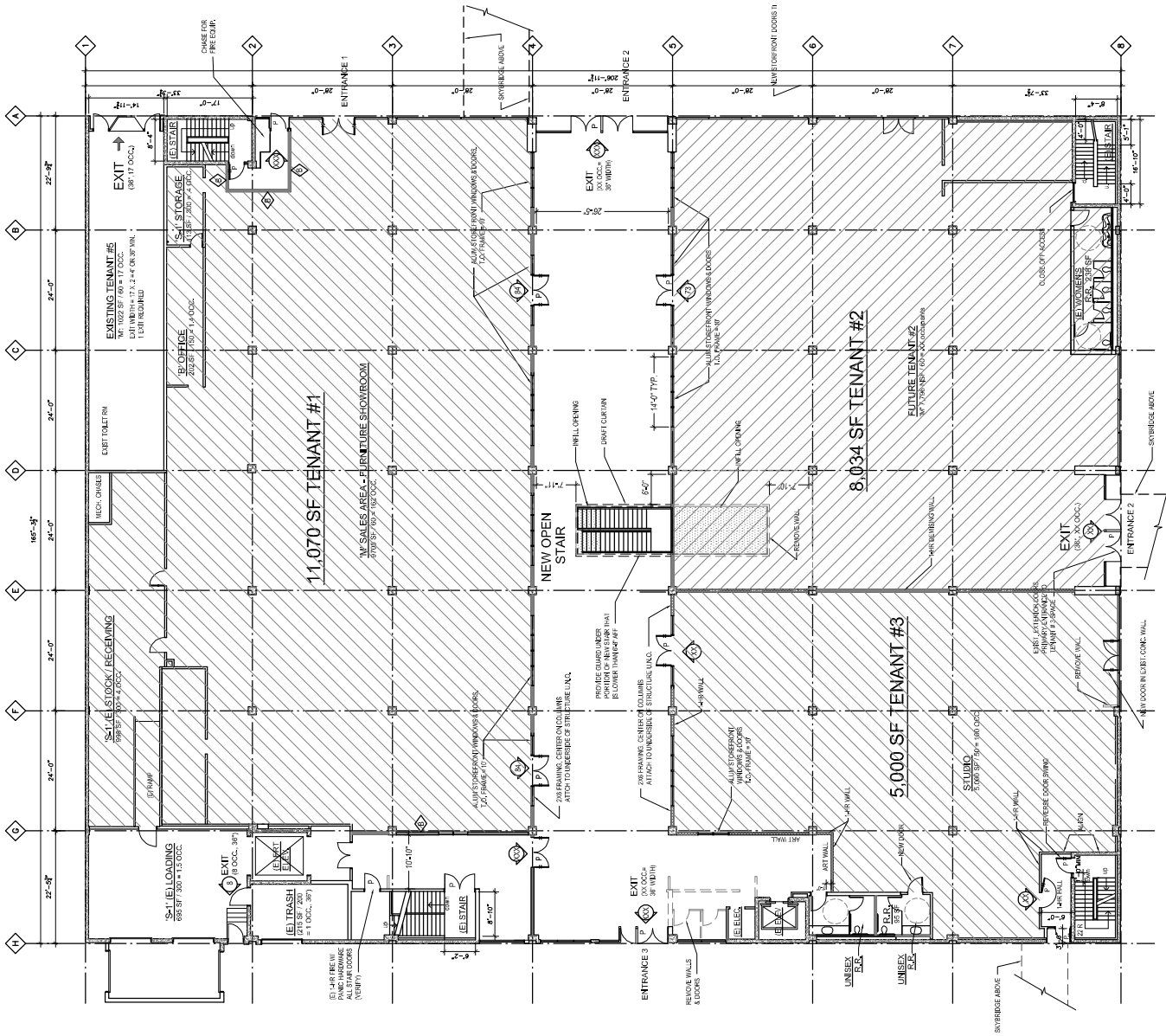
1 FLOOR PLAN - FIRST FLOOR REVISION TO PERMIT
