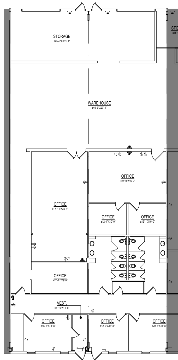
UNIT 15-18 PLANS SCALE: 1/16" = 1'-0"
