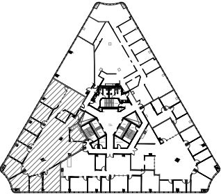
KEYPLAN - 5TH FLOOR
