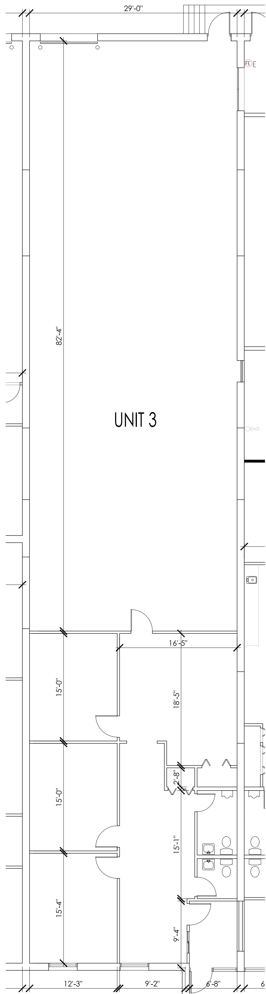
1 EXISTING OFFICE PLAN EC-1 SCALE: 1/8" = 1'-0"
