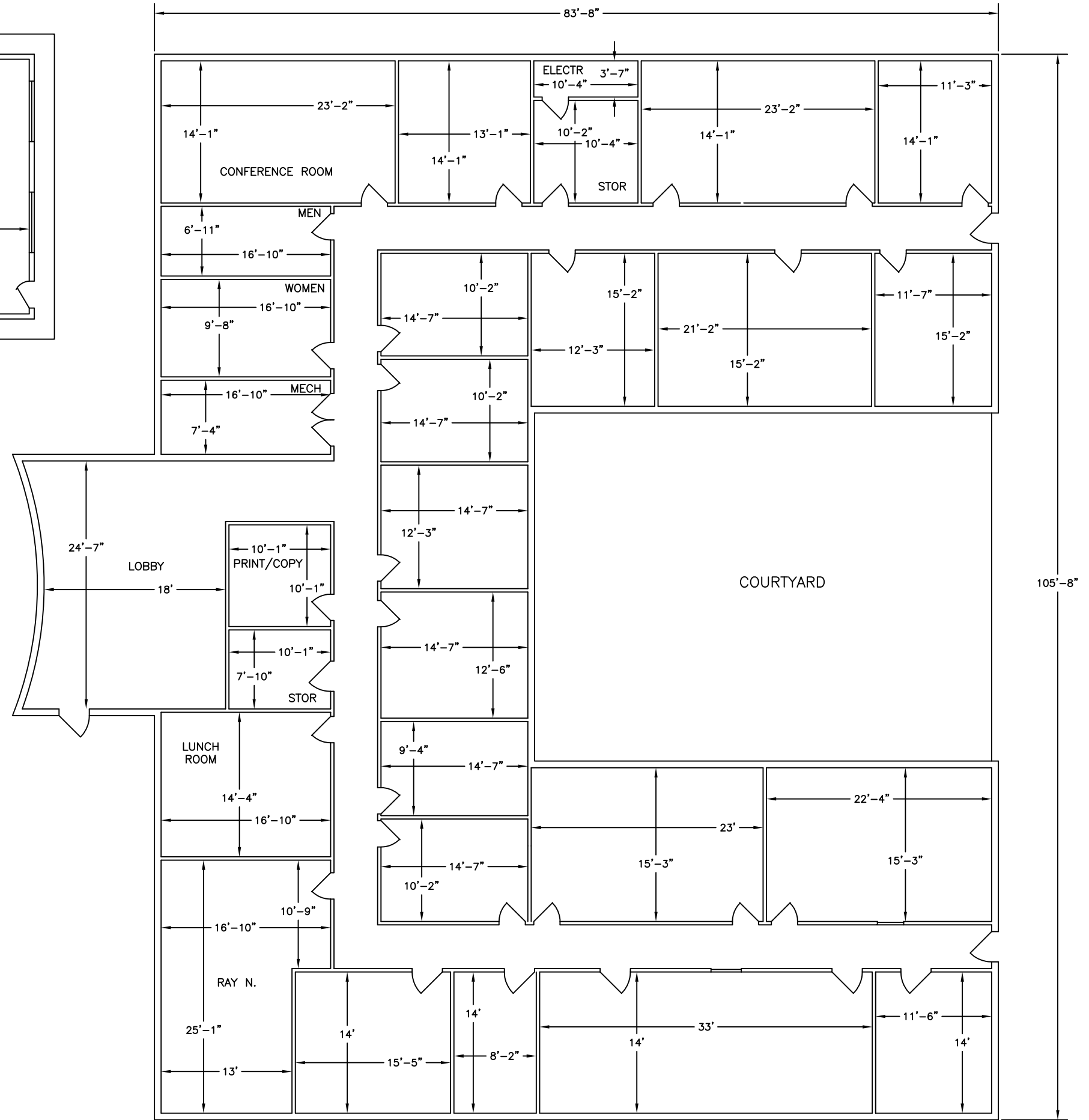
FIRST FLOOR
