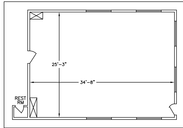
SECOND FLOOR
