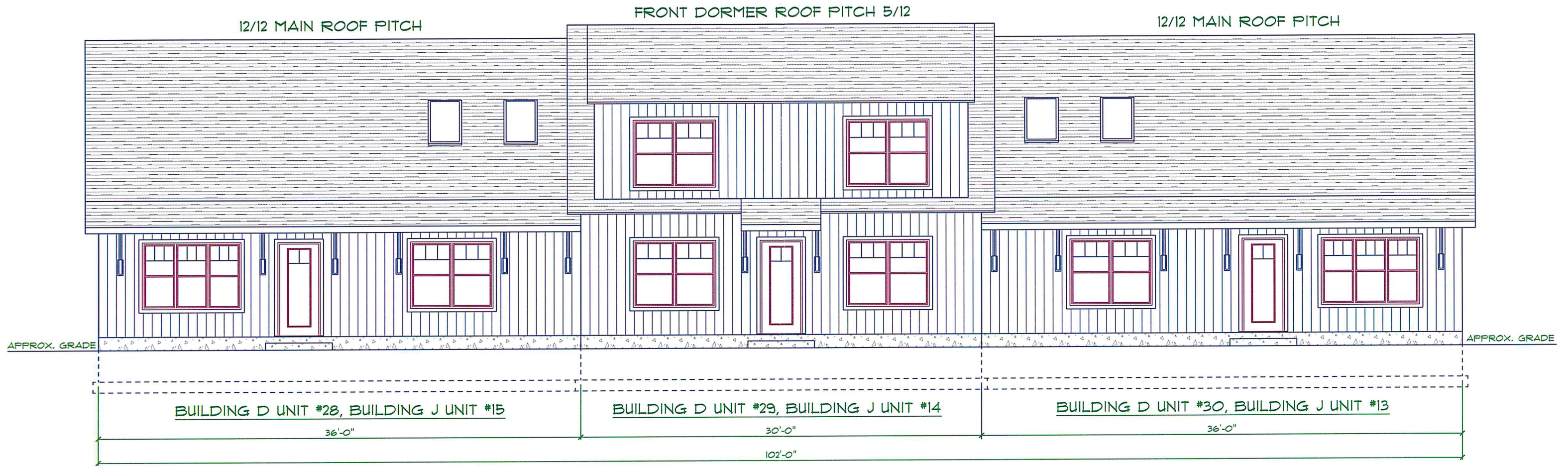
BUILDING J UNIT #13, UNIT #14, & UNIT #15 FRONT ELEVATION
