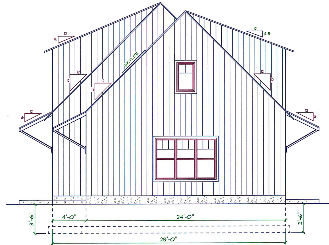
BUILDING J RIGHT SIDE ELEVATION ROCKY CORNER, BETHANY, CT
