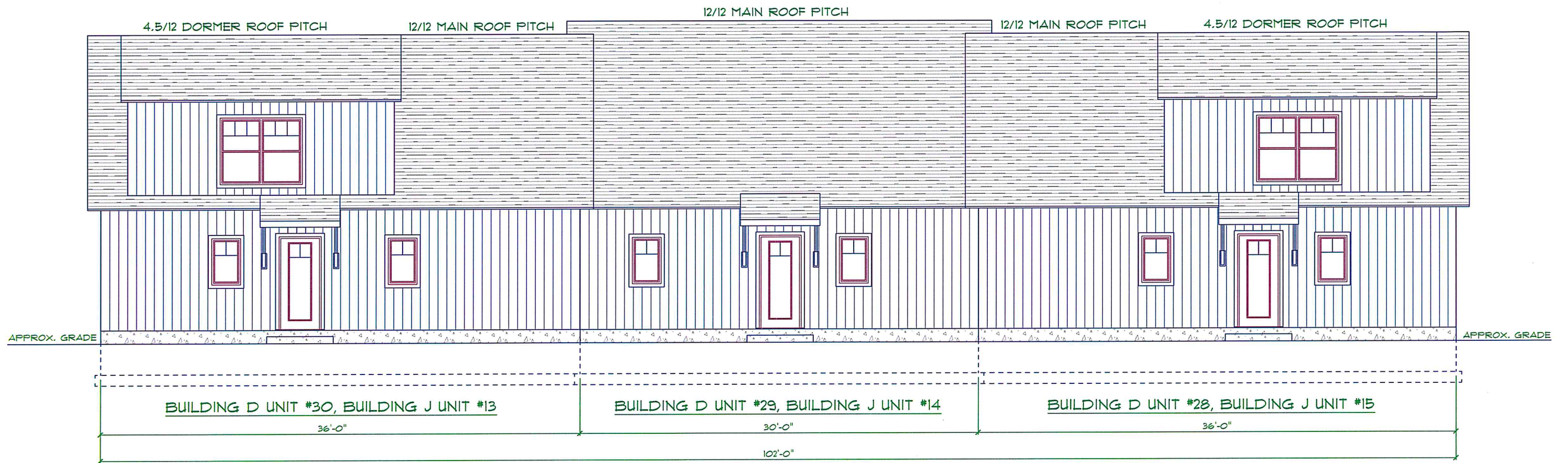
BUILDING J UNIT #13, UNIT #14, & UNIT #15 REAR ELEVATION ROCKY CORNER, BETHANY, CT
