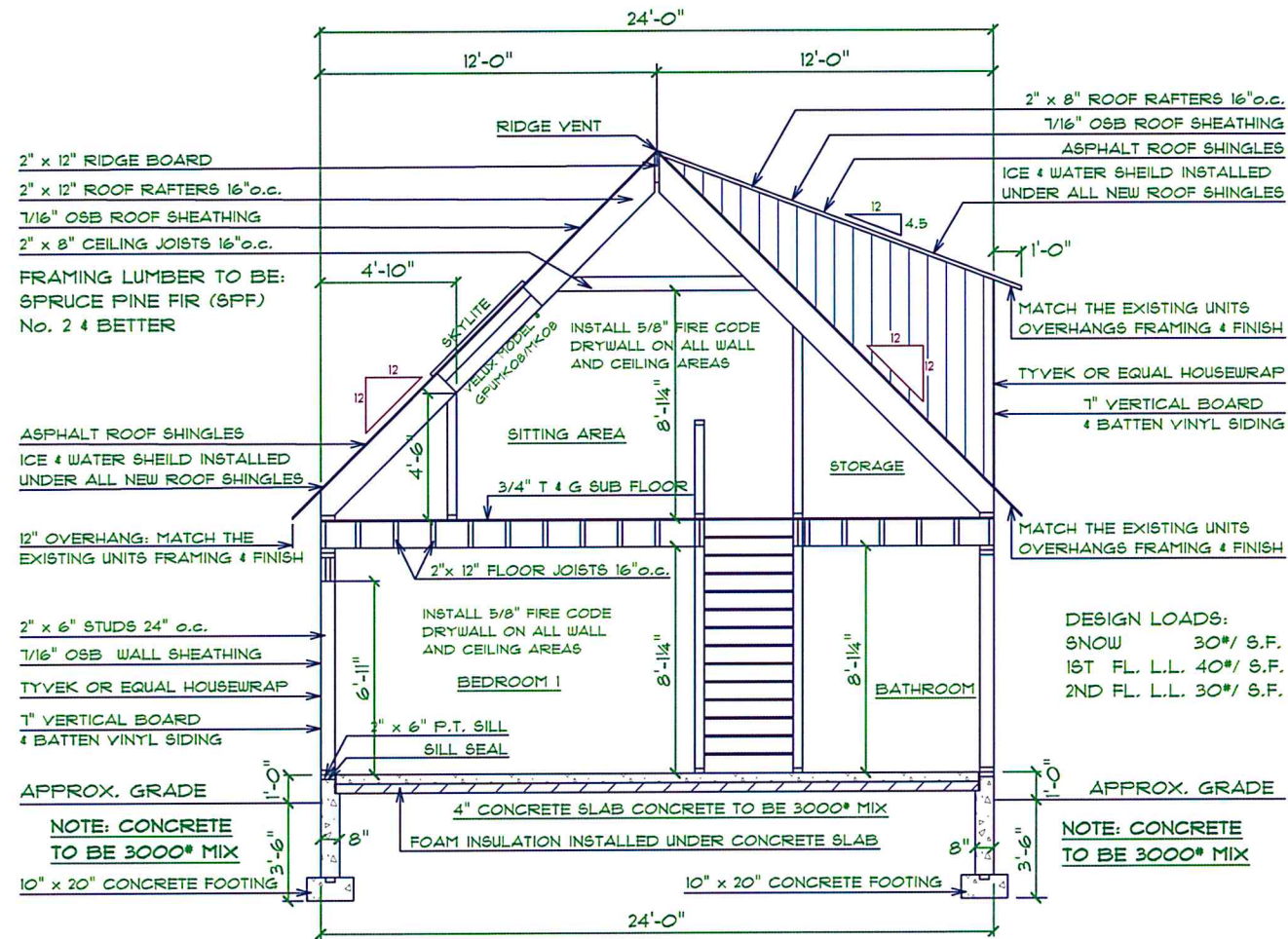
BUILDING J UNITS 13 & 15 CROSS SECTION I ROCKY CORNER, BETHANY, CT
