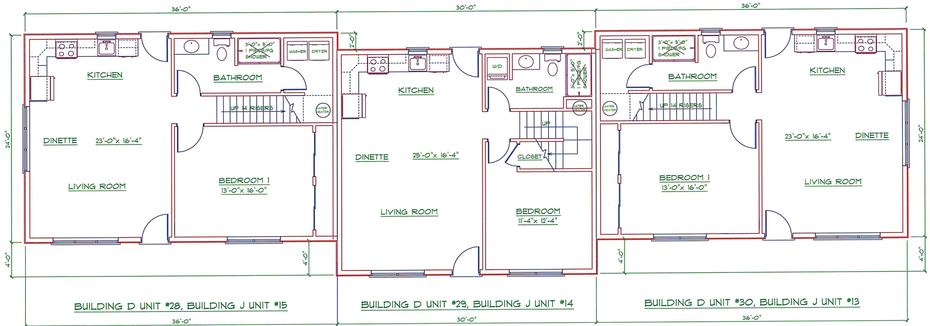
BUILDING J UNIT #13, UNIT #14, & UNIT #15 FIRST FLOOR PLAN
