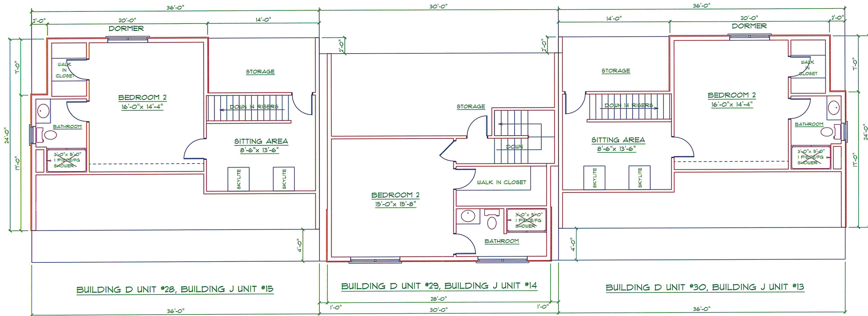
BUILDING J UNIT #13, UNIT #14, & UNIT #15 SECOND FLOOR PLAN
