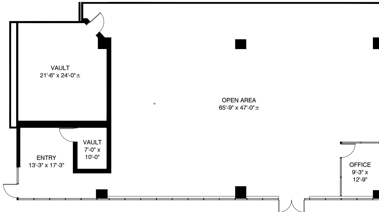
KEYPLAN - 1ST FLOOR
