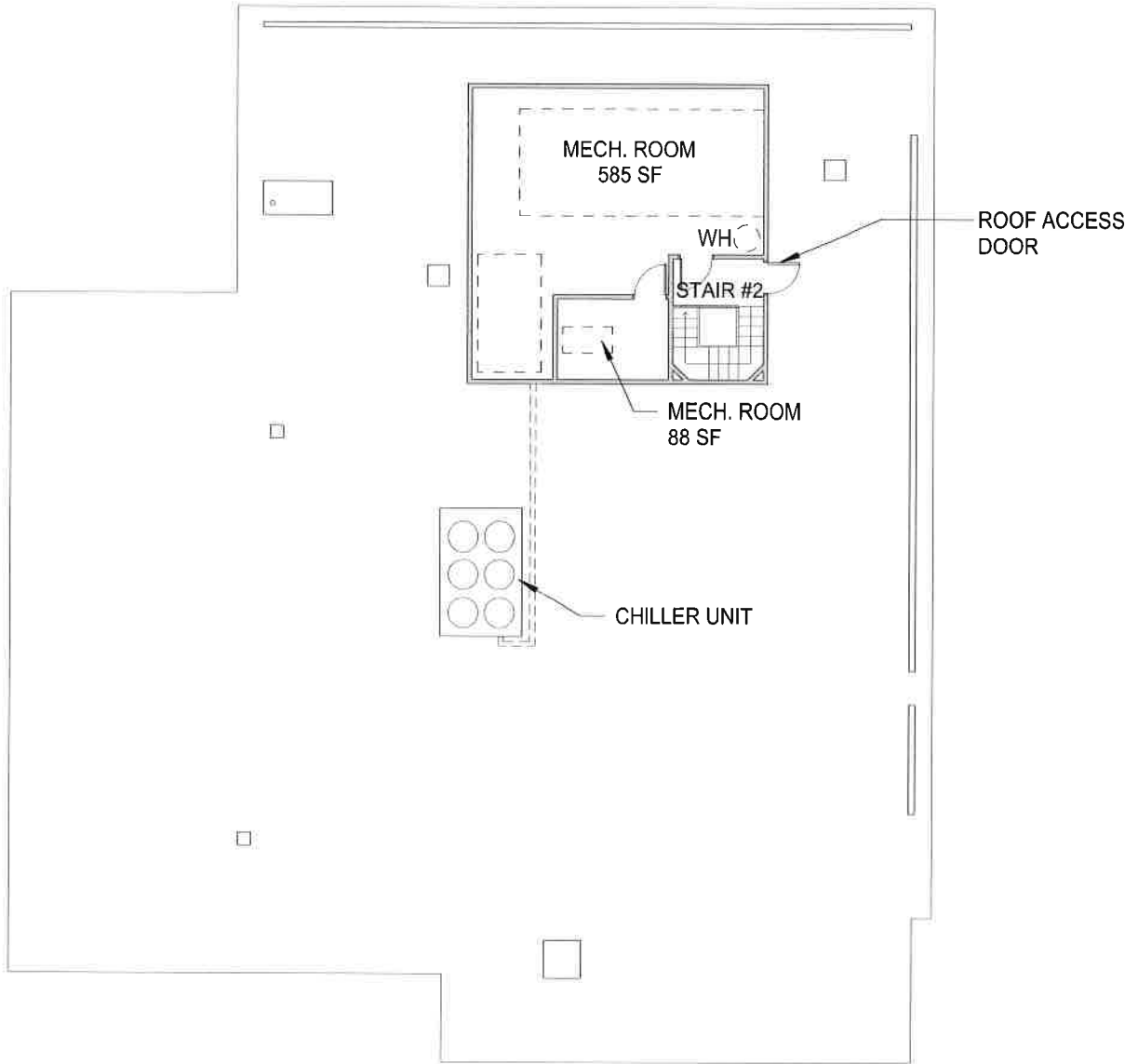
1 ROOF PLAN - Existing SCALE: 1/16" = 1'-0" 0 4' 8' 16'
