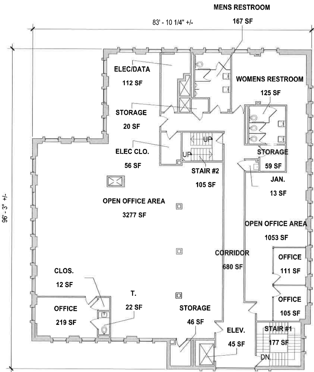
1 2ND FLOOR PLAN - EXISTING SCALE: 1/16" = 1'-0"
