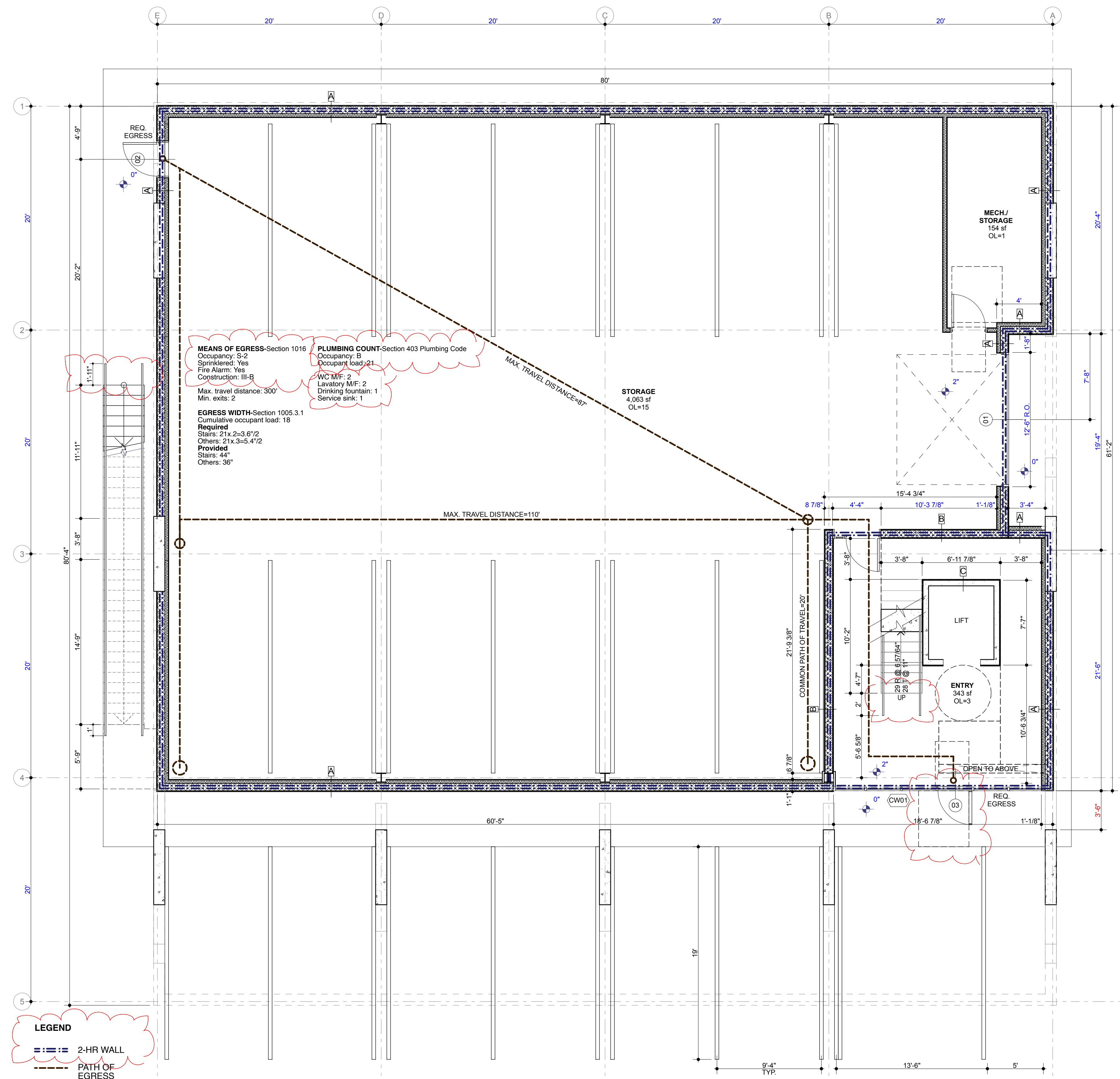
ground level life safety plan scale: 3/16" = 1'-0"
