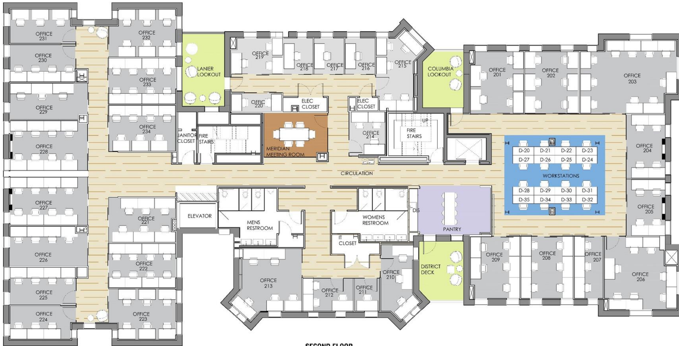
SECOND FLOOR
