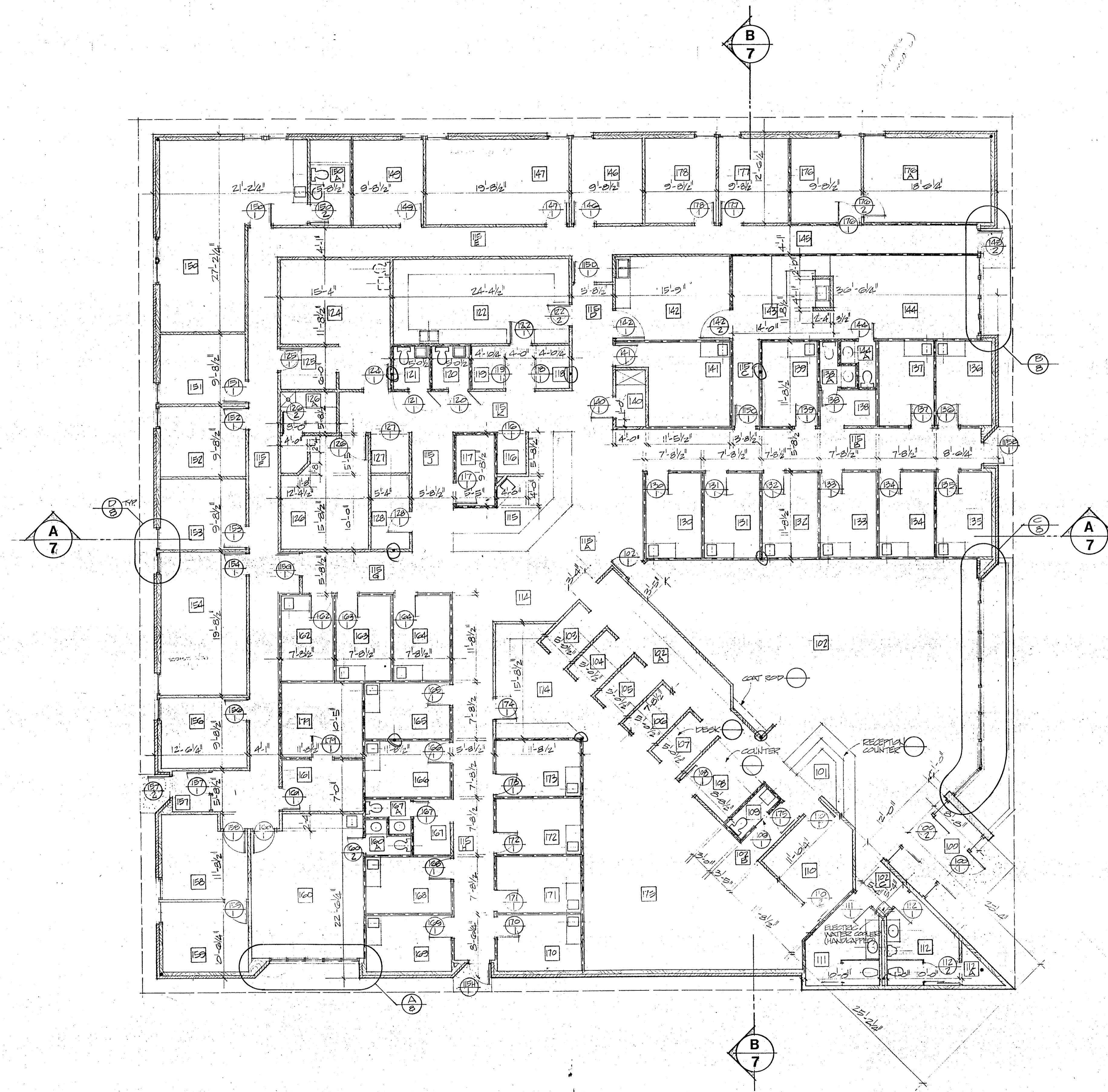
FLOOR PLAN 1/8" = 1'-0"
