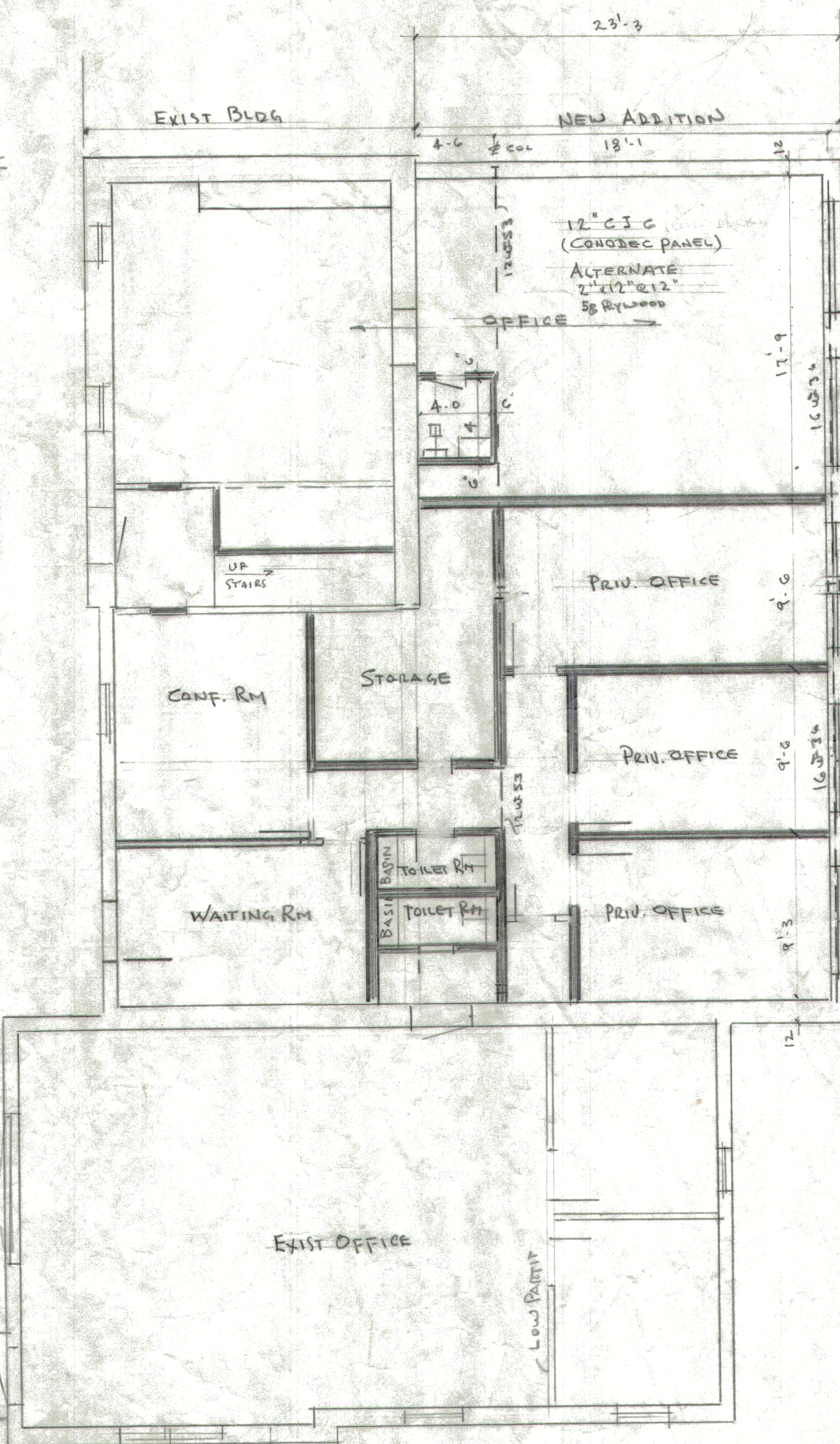
1ST FLOOR
