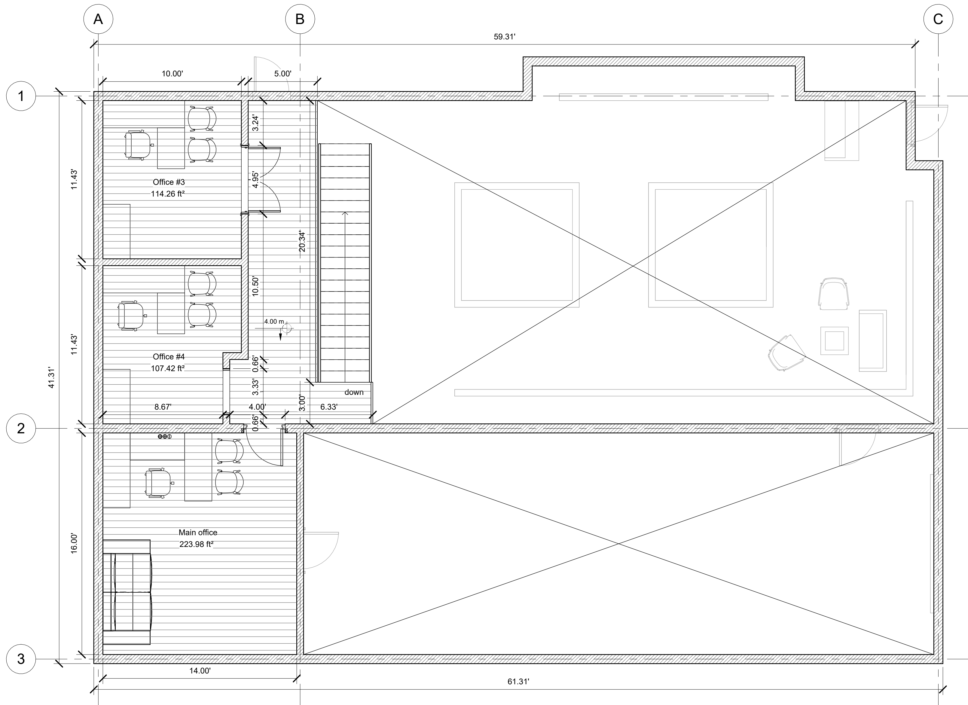
A2 2nd Level Floor Plan 1 : 50
