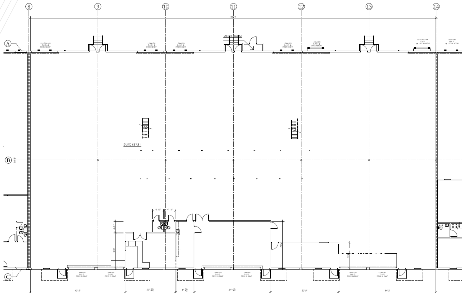
FLOOR PLAN
