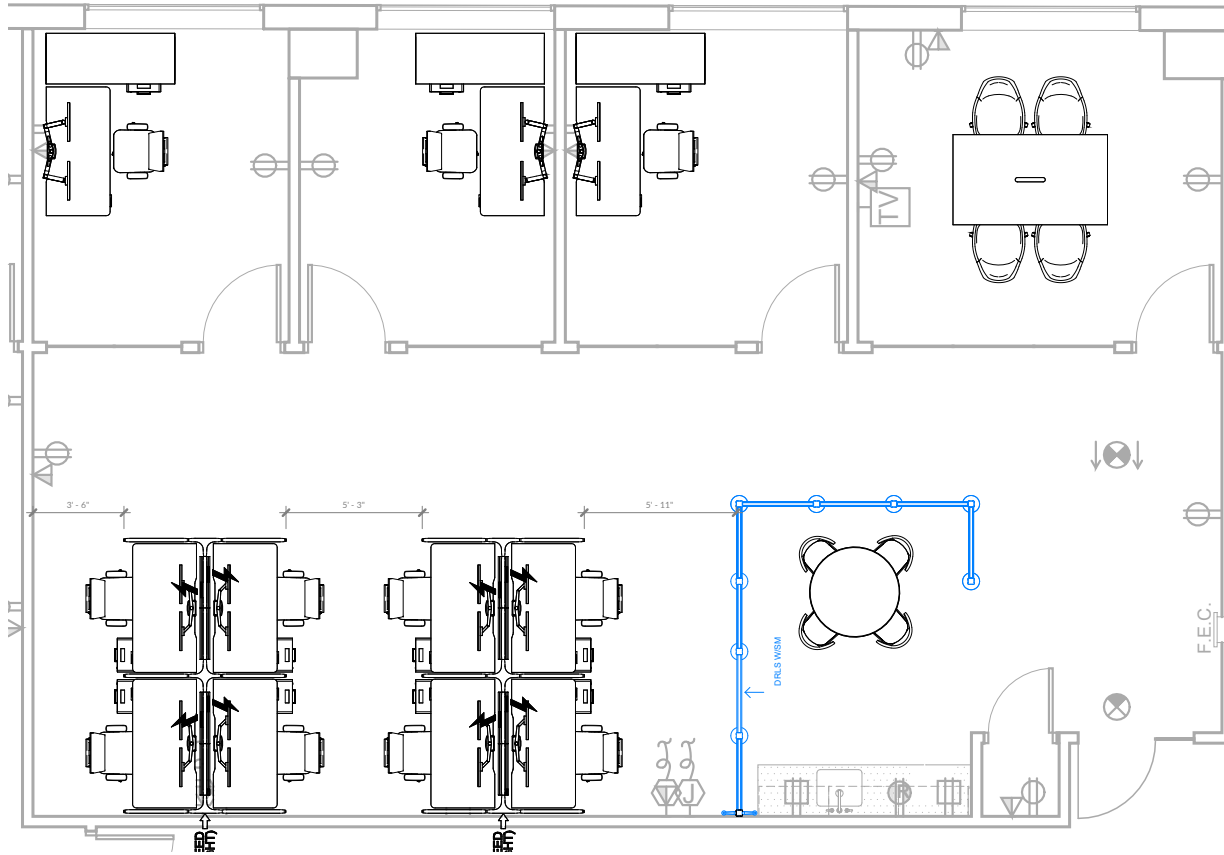
HYPOTHETICAL FURNITURE PLAN
