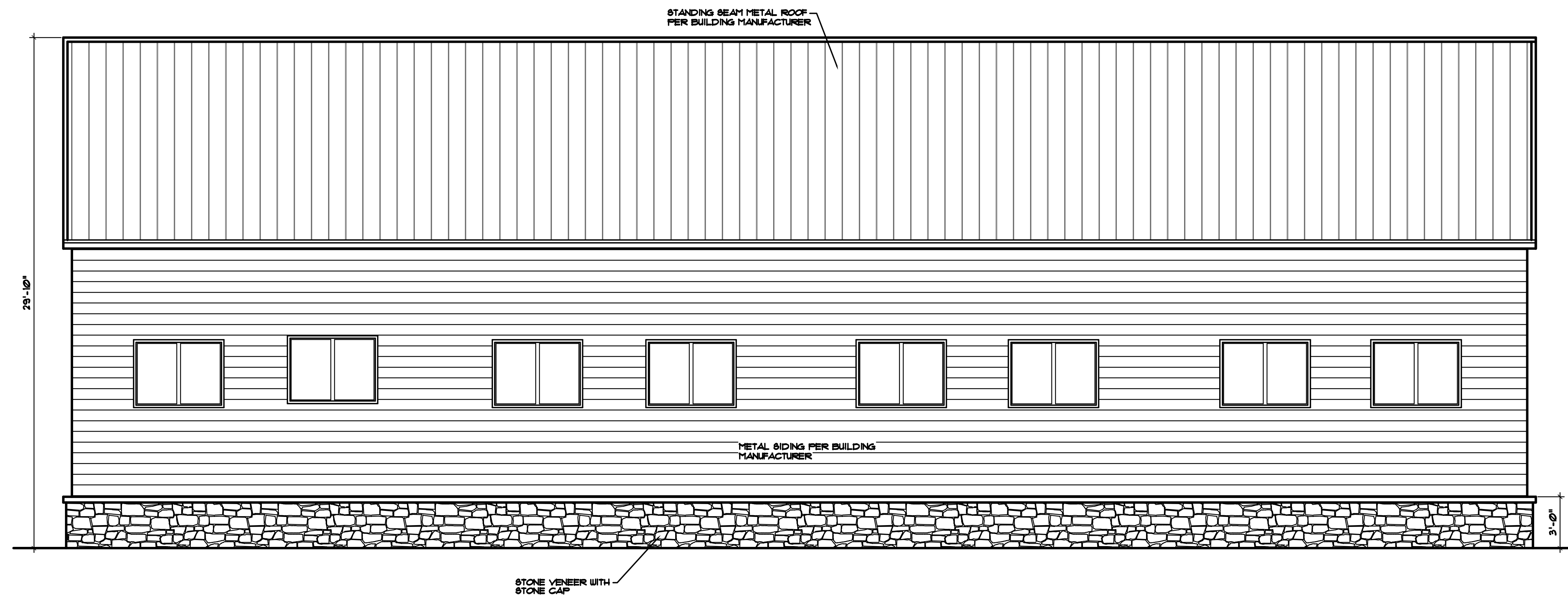
FRONT (STREET SIDE) ELEVATION SCALE 1/4"=1'-0"
