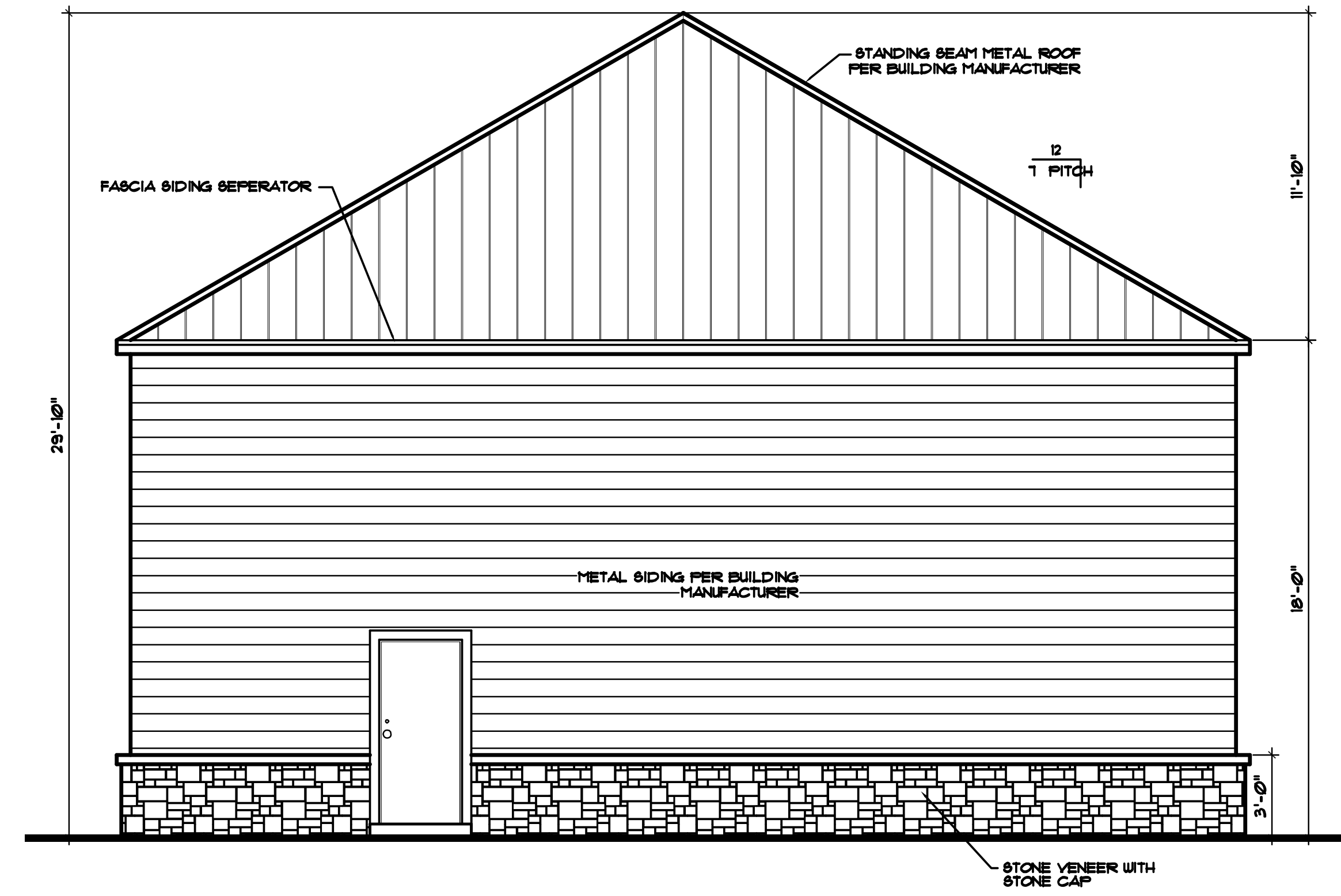
RIGHT END ELEVATION SCALE 1/4"=1'-0"
