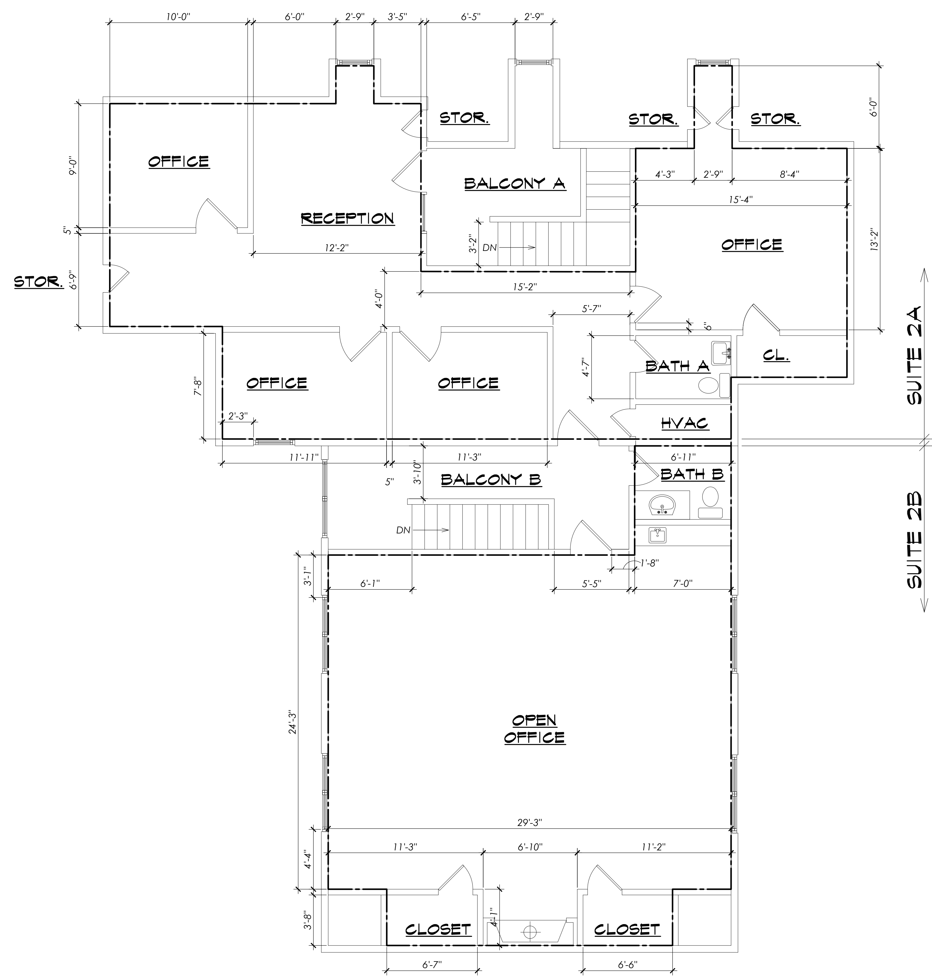
EXISTING FLOOR PLAN SUITES 2A & 2B SCALE: 1/4" = 1'-0"
