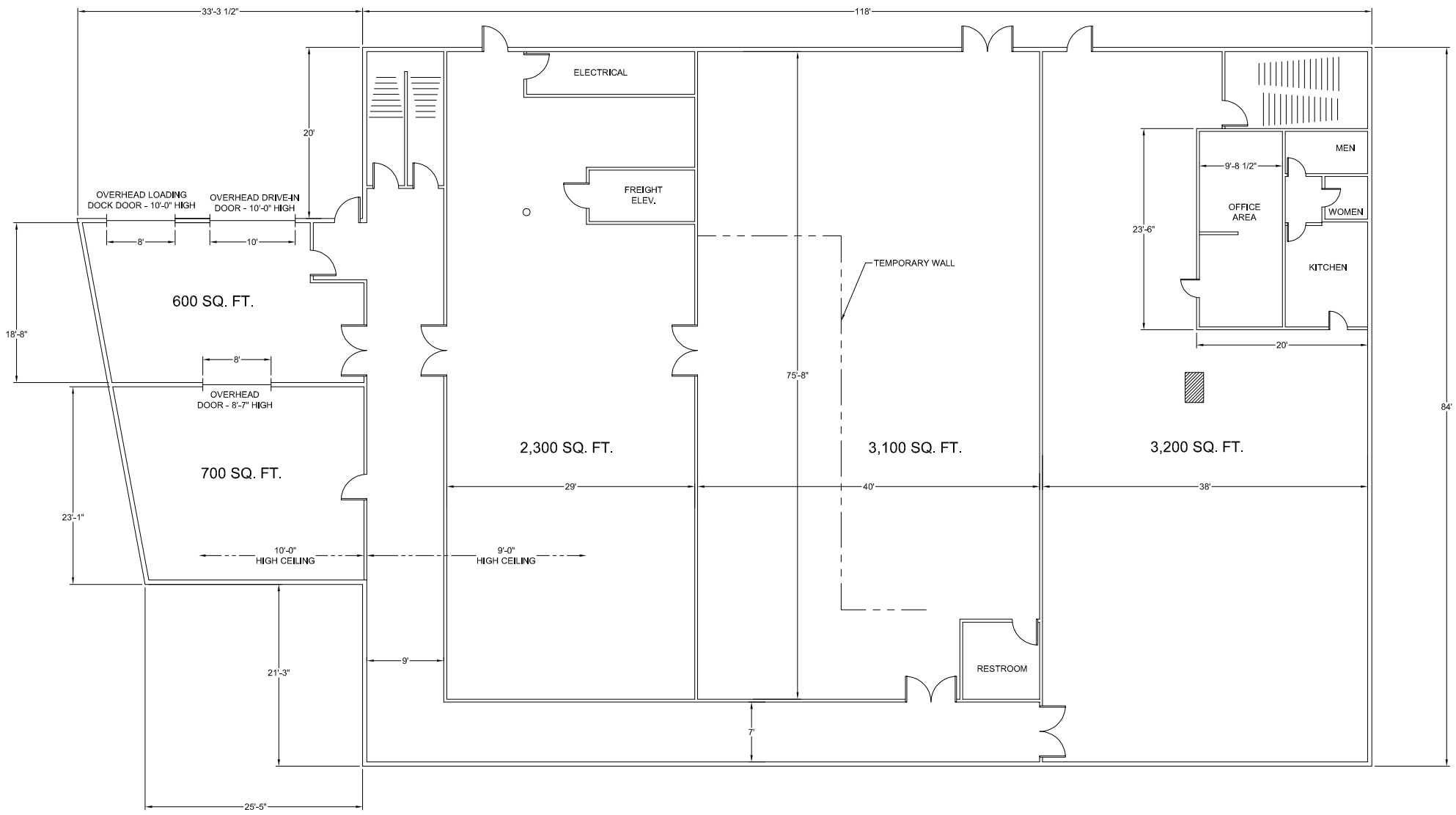
2nd LOWER LEVEL PLAN VIEW
