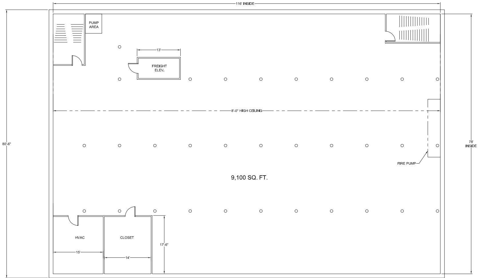
BASEMENT LEVEL PLAN VIEW
